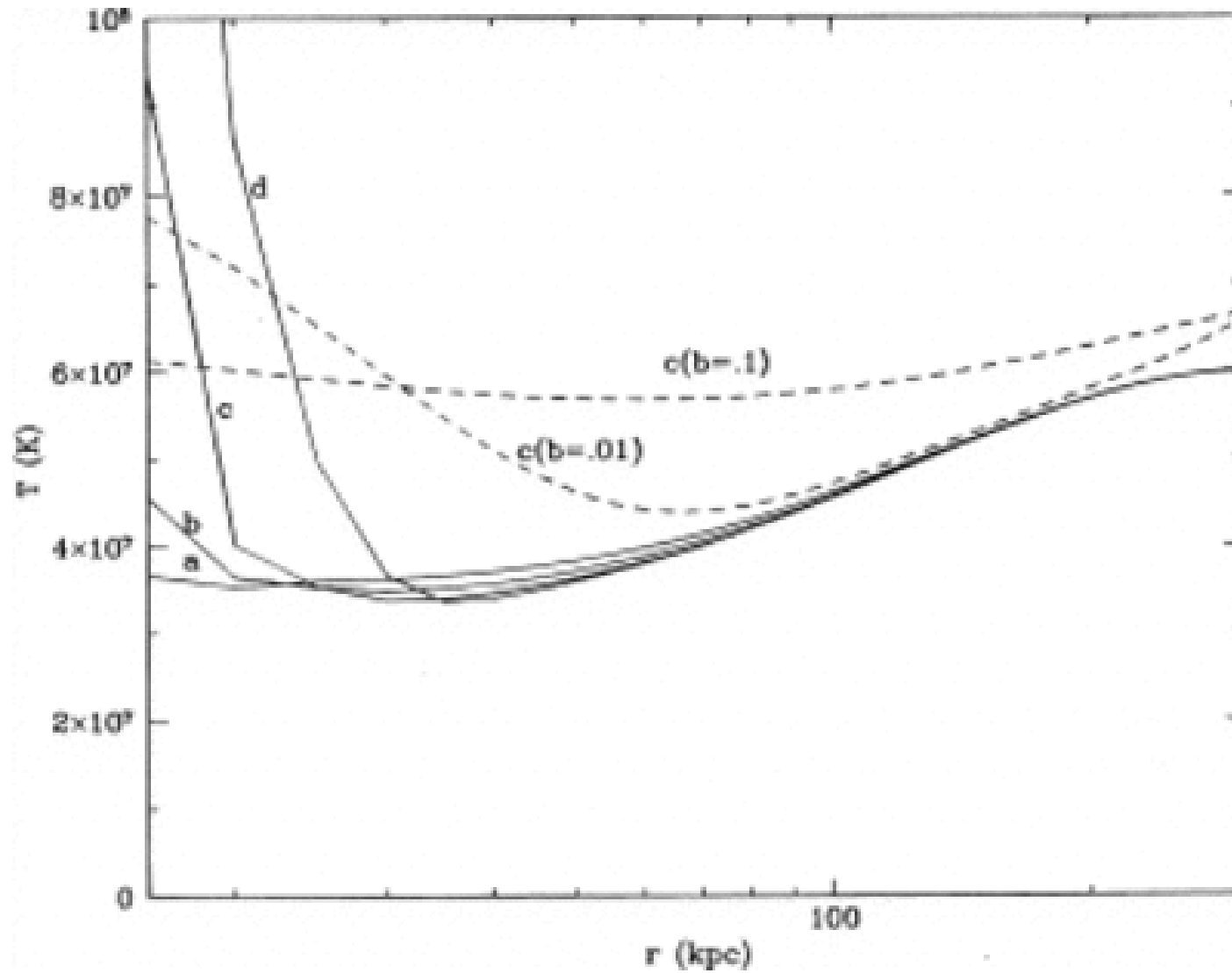
Fig. 4. from A Feedback Model for Radio Sources Fueled by Cooling Flows Tucker & David 1997 ApJ 484 602 doi:10.1086/304345 https://dx.doi.org/10.1086/304345 © 1997. The American Astronomical Society. All rights reserved. Printed in U.S.A.
