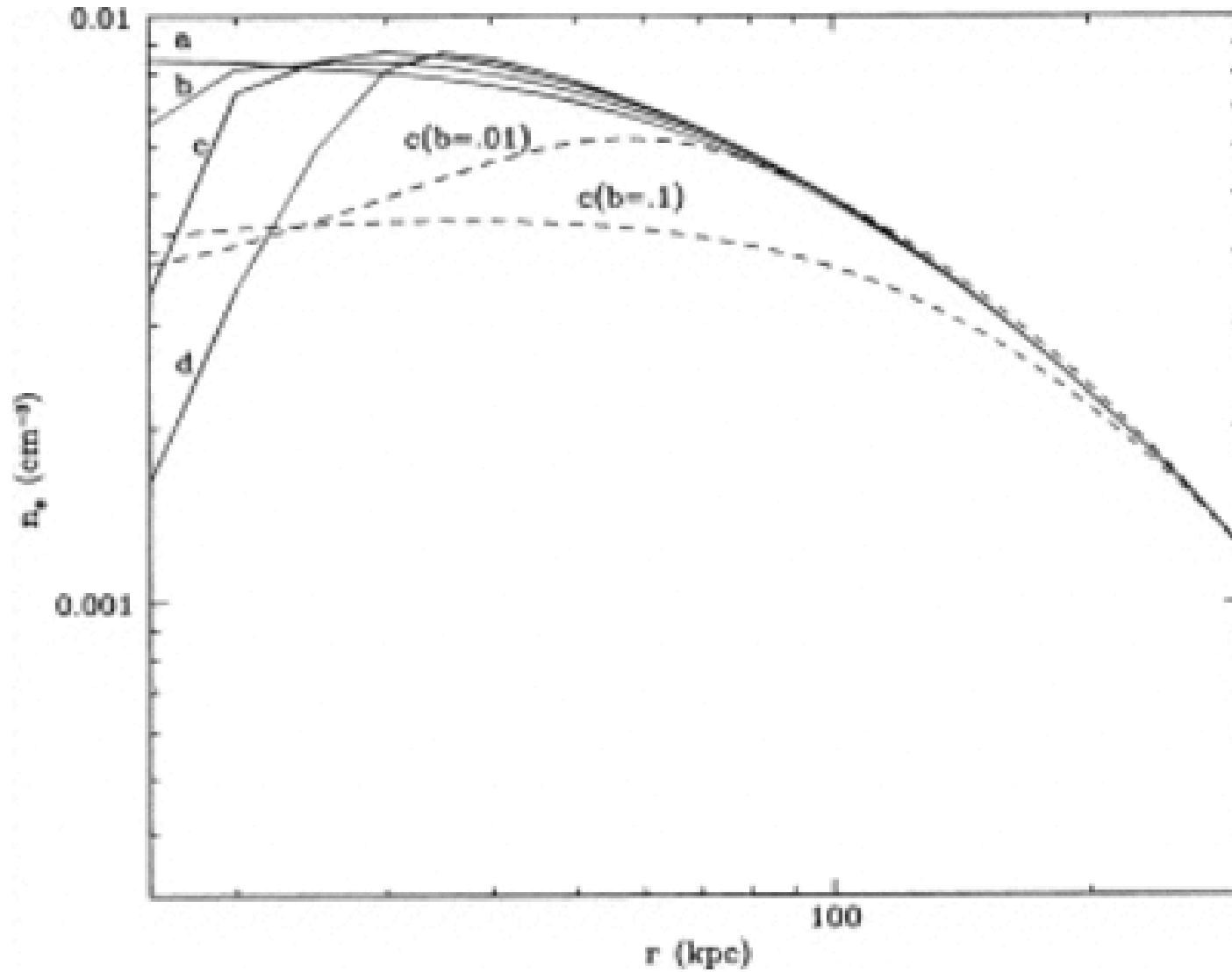
Fig. 3. from A Feedback Model for Radio Sources Fueled by Cooling Flows Tucker & David 1997 ApJ 484 602 doi:10.1086/304345 https://dx.doi.org/10.1086/304345 © 1997. The American Astronomical Society. All rights reserved. Printed in U.S.A.
