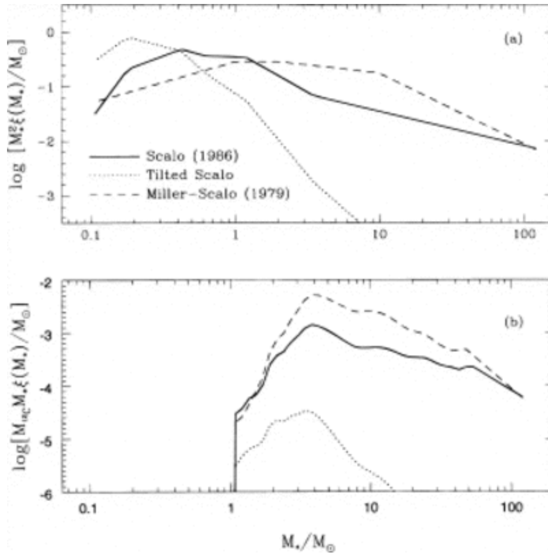
Fig. 9. from Signatures of Stellar Reionization of the Universe Haiman & Loeb 1997 ApJ 483 21 doi:10.1086/304238 https://dx.doi.org/10.1086/304238 © 1997. The American Astronomical Society. All rights reserved. Printed in U.S.A.
