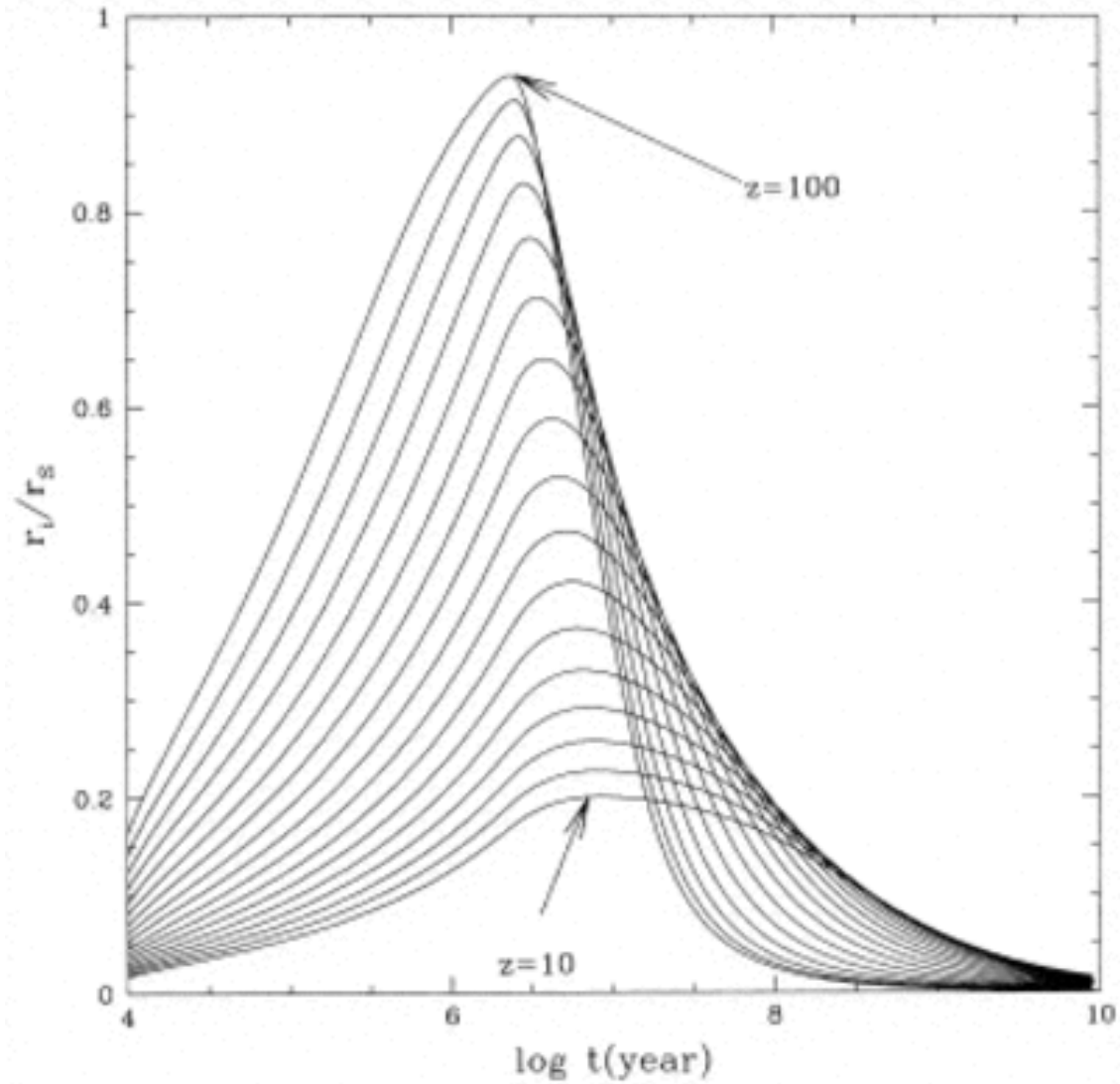
Fig. 7. from Signatures of Stellar Reionization of the Universe Haiman & Loeb 1997 ApJ 483 21 doi:10.1086/304238 https://dx.doi.org/10.1086/304238 © 1997. The American Astronomical Society. All rights reserved. Printed in U.S.A.
