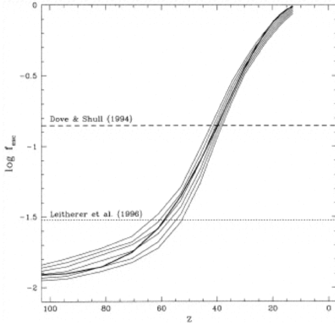
Fig. 6. from Signatures of Stellar Reionization of the Universe Haiman & Loeb 1997 ApJ 483 21 doi:10.1086/304238 https://dx.doi.org/10.1086/304238 © 1997. The American Astronomical Society. All rights reserved. Printed in U.S.A.
