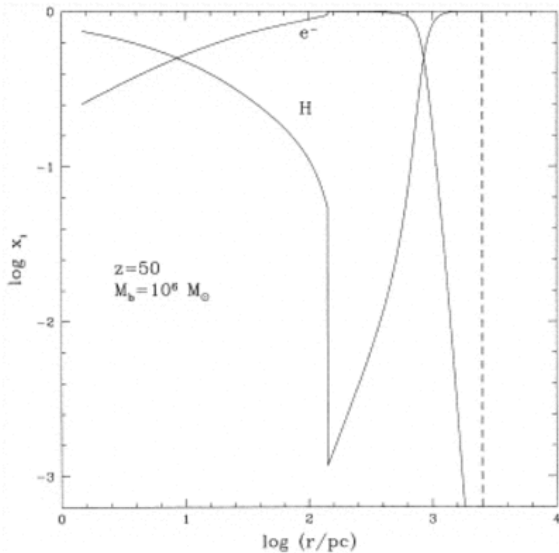
Fig. 5. from Signatures of Stellar Reionization of the Universe Haiman & Loeb 1997 ApJ 483 21 doi:10.1086/304238 https://dx.doi.org/10.1086/304238 © 1997. The American Astronomical Society. All rights reserved. Printed in U.S.A.
