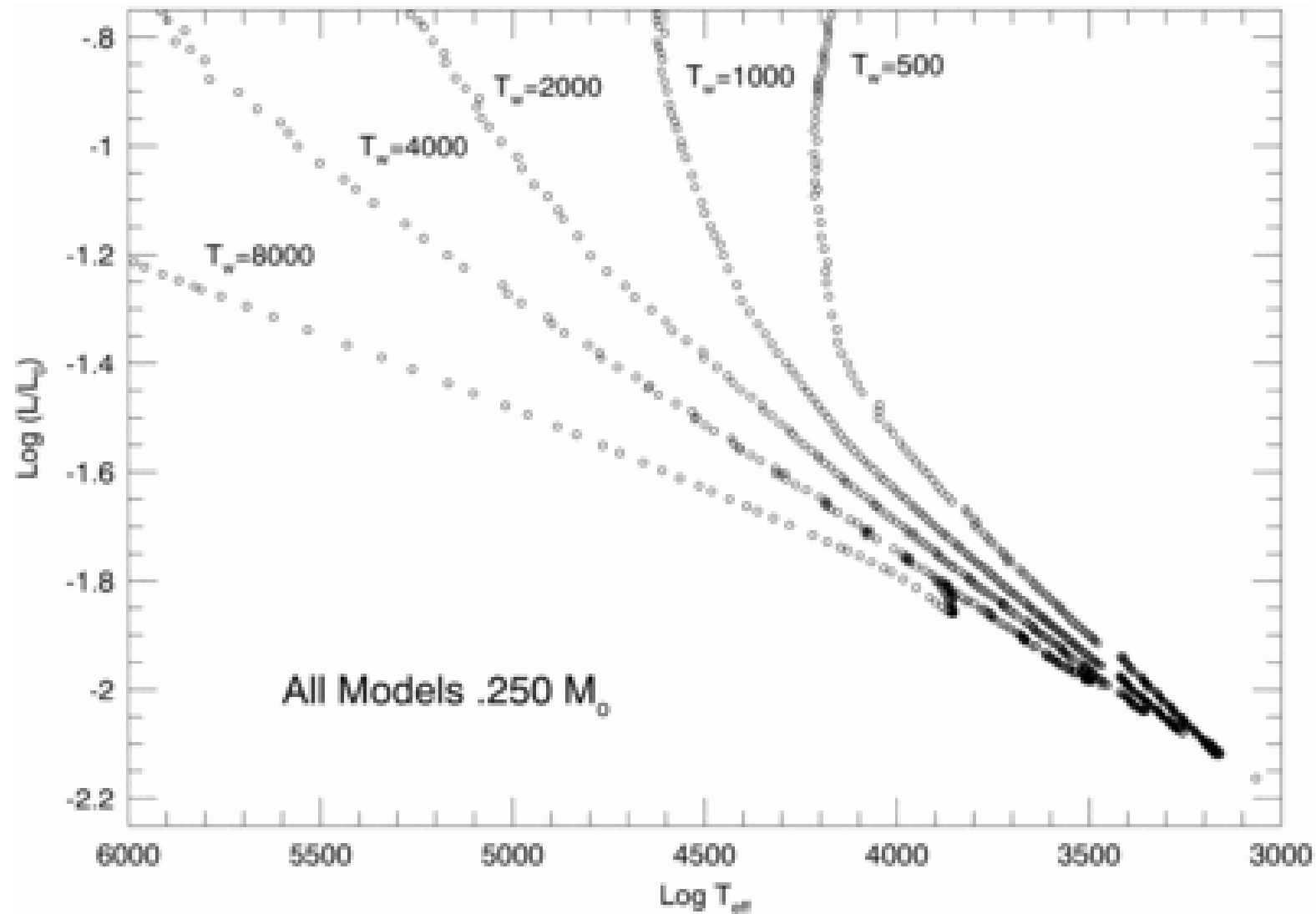
Fig. 7. from The End of the Main Sequence Laughlin, Bodenheimer, & Adams 1997 ApJ 482 420 doi:10.1086/304125 https://dx.doi.org/10.1086/304125 © 1997. The American Astronomical Society. All rights reserved. Printed in U.S.A.
