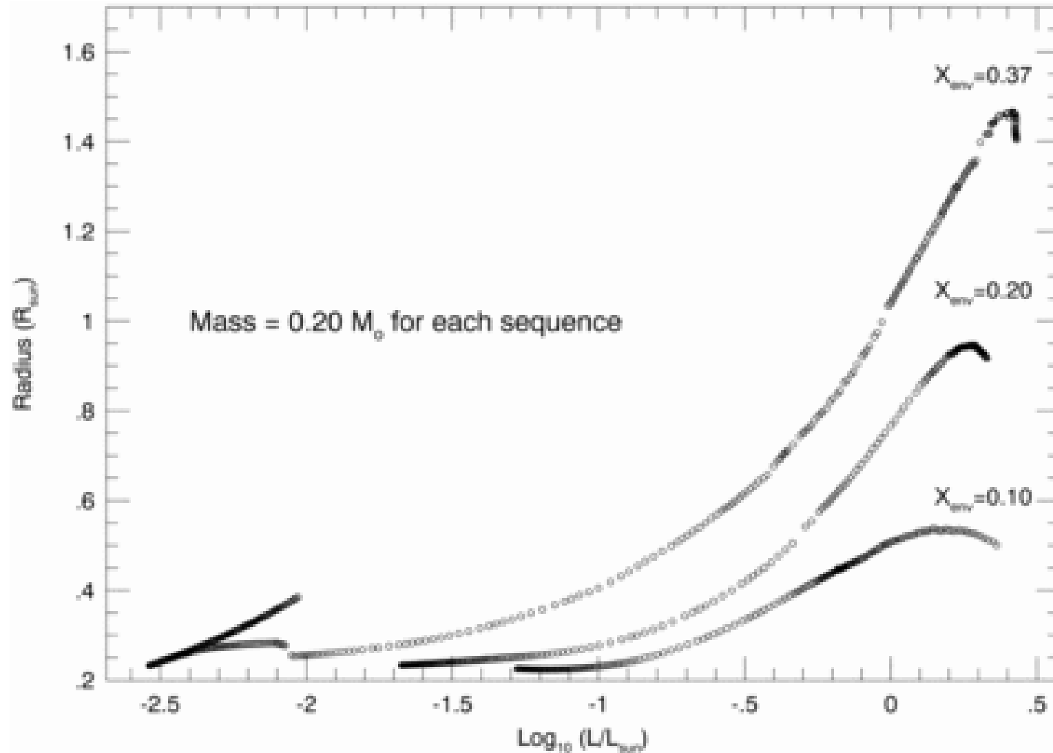
Fig. 5. from The End of the Main Sequence Laughlin, Bodenheimer, & Adams 1997 ApJ 482 420 doi:10.1086/304125 https://dx.doi.org/10.1086/304125 © 1997. The American Astronomical Society. All rights reserved. Printed in U.S.A.
