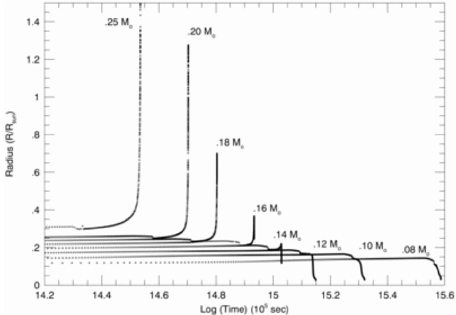
Fig. 4. from The End of the Main Sequence Laughlin, Bodenheimer, & Adams 1997 ApJ 482 420 doi:10.1086/304125 https://dx.doi.org/10.1086/304125 © 1997. The American Astronomical Society. All rights reserved. Printed in U.S.A.
