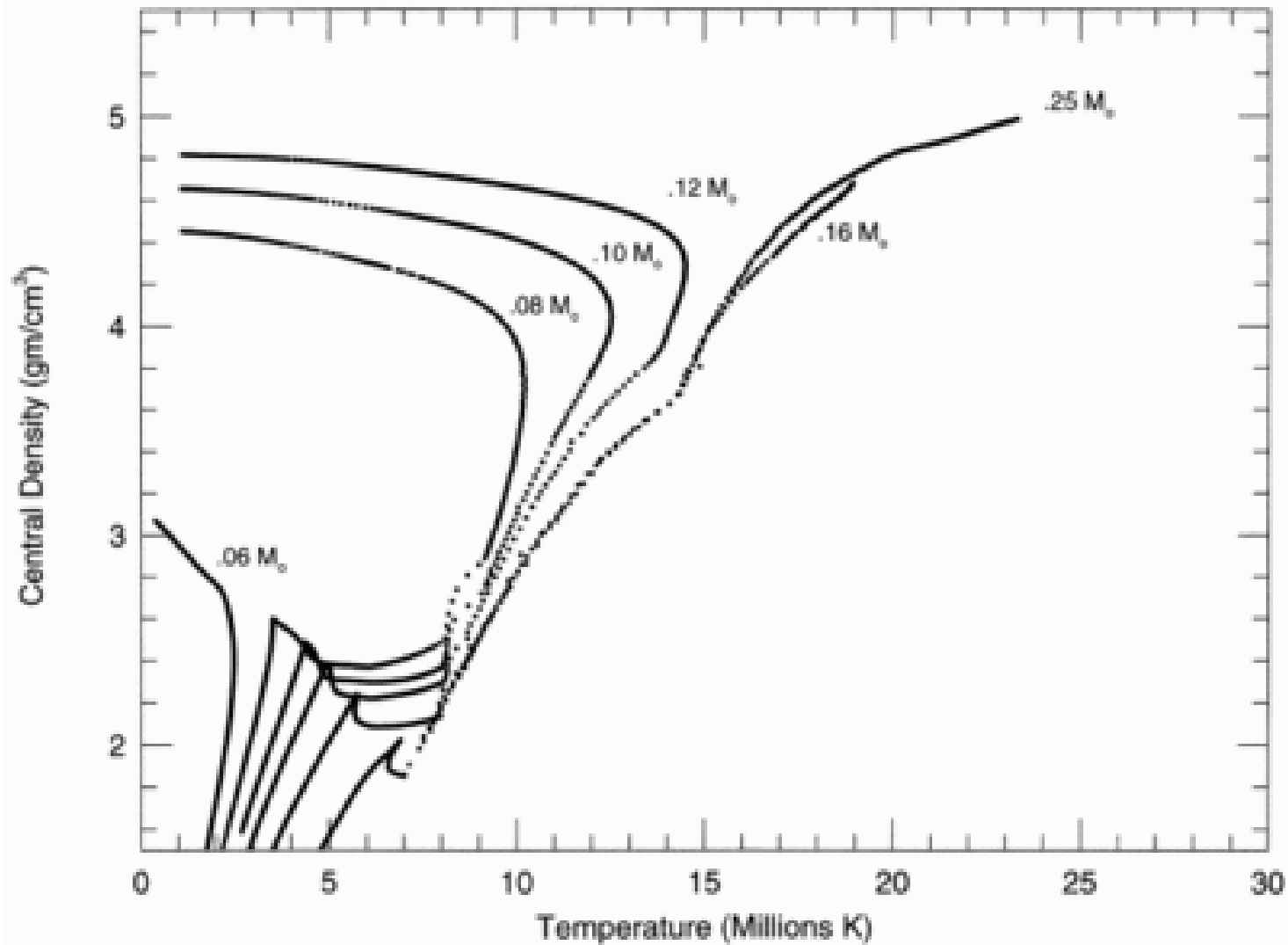
Fig. 3. from The End of the Main Sequence Laughlin, Bodenheimer, & Adams 1997 ApJ 482 420 doi:10.1086/304125 https://dx.doi.org/10.1086/304125 © 1997. The American Astronomical Society. All rights reserved. Printed in U.S.A.
