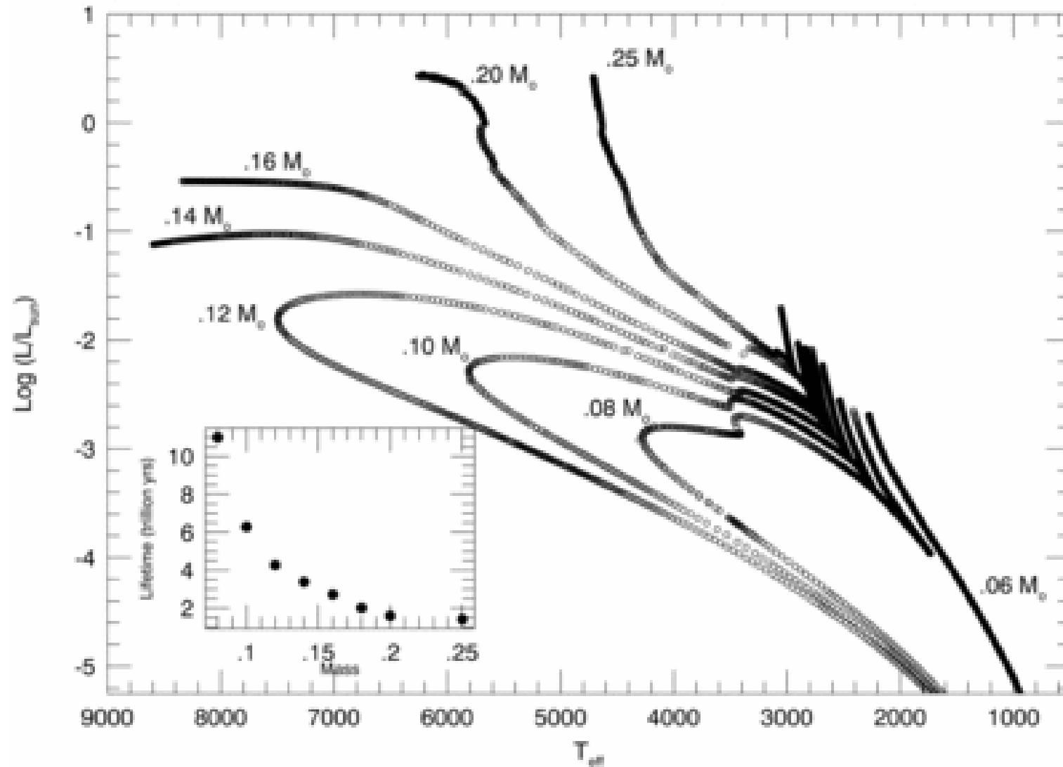
Fig. 2. from The End of the Main Sequence Laughlin, Bodenheimer, & Adams 1997 ApJ 482 420 doi:10.1086/304125 https://dx.doi.org/10.1086/304125 © 1997. The American Astronomical Society. All rights reserved. Printed in U.S.A.
