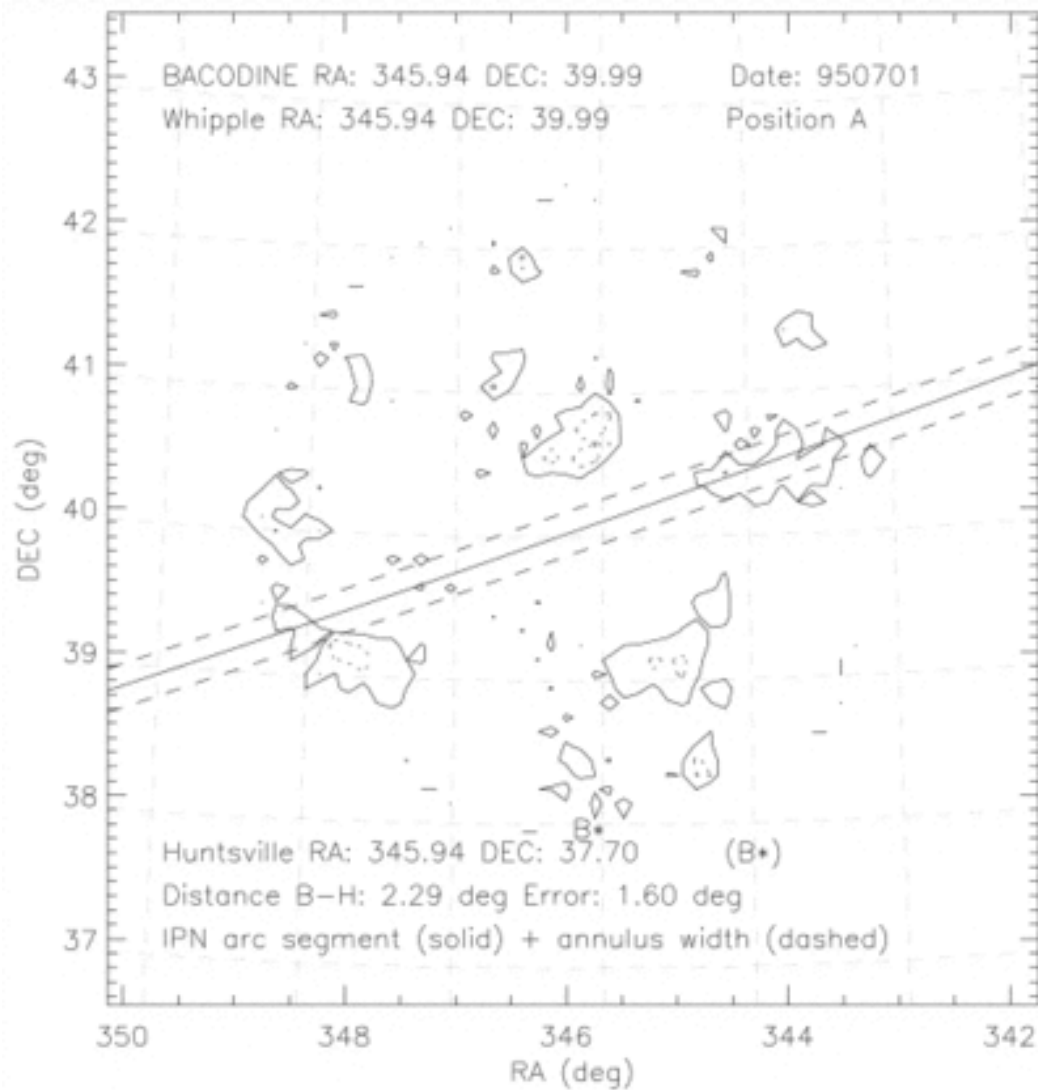
Fig. 5. from A Search for TeV Counterparts to BATSE GammaRay Bursts Connaughton et al. 1997 ApJ 479 859 doi:10.1086/303918 https://dx.doi.org/10.1086/303918 © 1997. The American Astronomical Society. All rights reserved. Printed in U.S.A.
