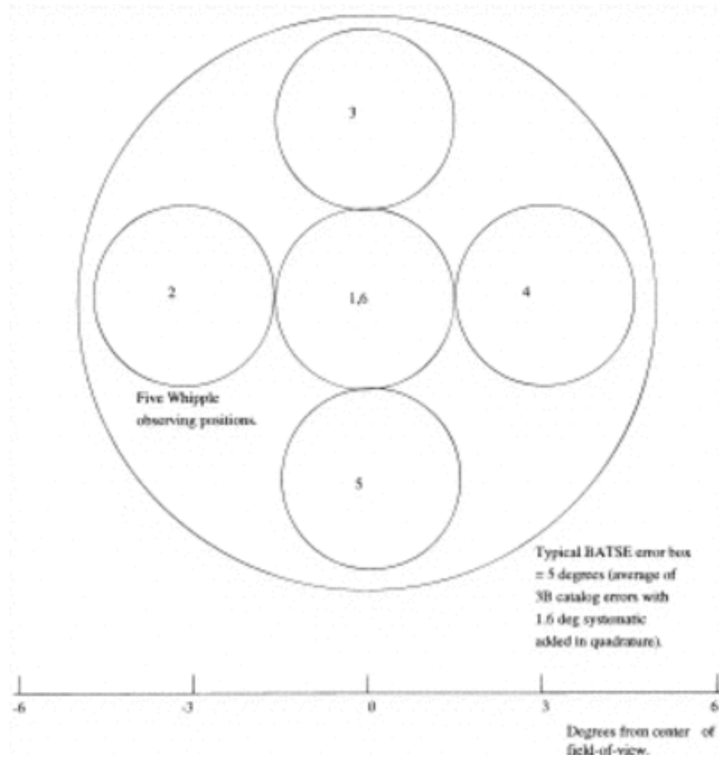
Fig. 1. from A Search for TeV Counterparts to BATSE GammaRay Bursts Connaughton et al. 1997 ApJ 479 859 doi:10.1086/303918 https://dx.doi.org/10.1086/303918 © 1997. The American Astronomical Society. All rights reserved. Printed in U.S.A.
