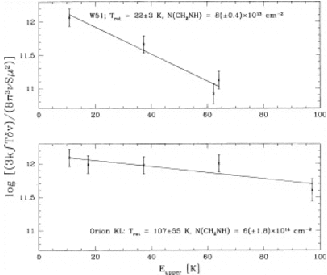
Fig. 2. from Hydrogenation of Interstellar Molecules: A Survey for Methyleneimine (CH 2 NH) Dickens et al. 1997 ApJ 479 307 doi:10.1086/303884 https://dx.doi.org/10.1086/303884 © 1997. The American Astronomical Society. All rights reserved. Printed in U.S.A.
