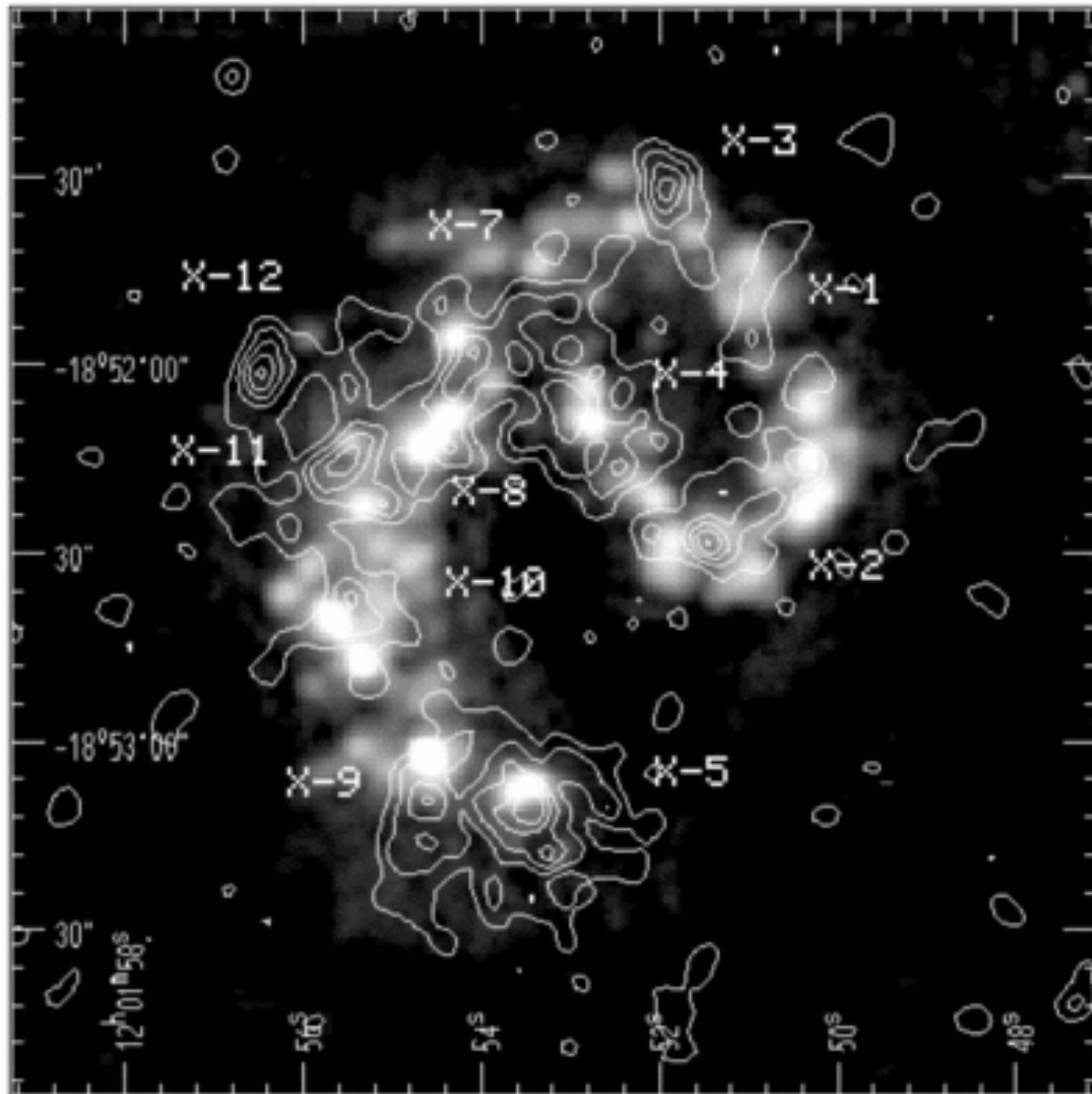
Fig. 5. from ROSAT HRI Observations of NGC 4038/4039, "The Antennae" Galaxies Fabbiano, Schweizer, & Mackie 1997 ApJ 478 542 doi:10.1086/303832 https://dx.doi.org/10.1086/303832 © 1997. The American Astronomical Society. All rights reserved. Printed in U.S.A.
