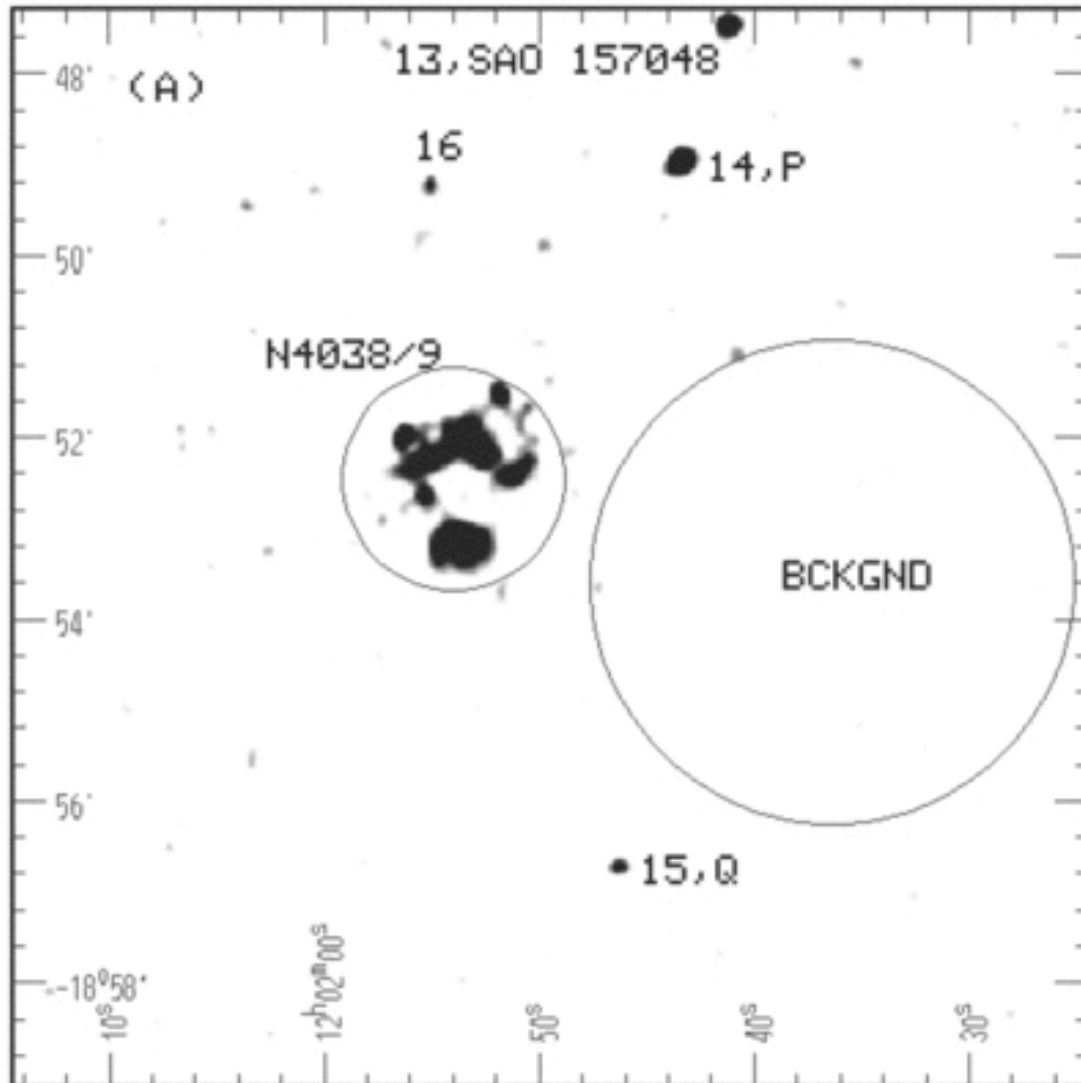
Fig. 3. from ROSAT HRI Observations of NGC 4038/4039, "The Antennae" Galaxies Fabbiano, Schweizer, & Mackie 1997 ApJ 478 542 doi:10.1086/303832 https://dx.doi.org/10.1086/303832 © 1997. The American Astronomical Society. All rights reserved. Printed in U.S.A.
