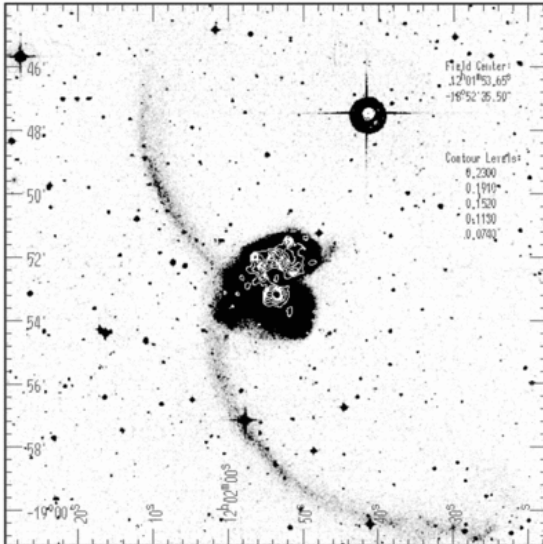
Fig. 1. from ROSAT HRI Observations of NGC 4038/4039, "The Antennae" Galaxies Fabbiano, Schweizer, & Mackie 1997 ApJ 478 542 doi:10.1086/303832 https://dx.doi.org/10.1086/303832 © 1997. The American Astronomical Society. All rights reserved. Printed in U.S.A.
