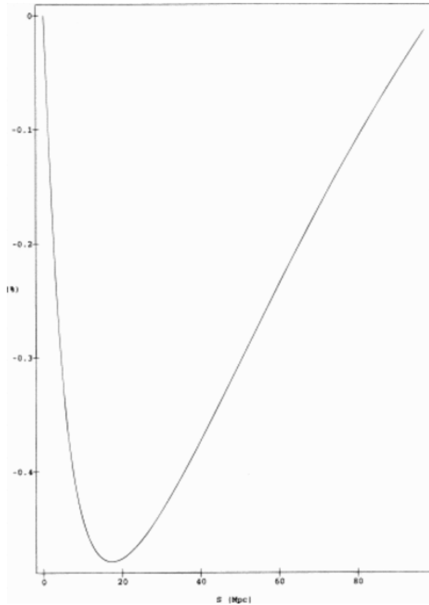
Fig. 3. from Anisotropic Observations in Universes with Nonlinear Inhomogeneity Humphreys, Maartens, & Matravers 1997 ApJ 477 47 doi:10.1086/303672 https://dx.doi.org/10.1086/303672 © 1997. The American Astronomical Society. All rights reserved. Printed in U.S.A.
