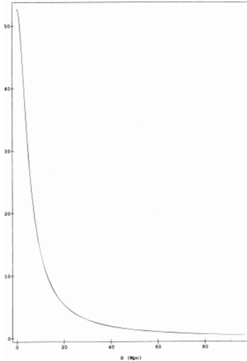
Fig. 2. from Anisotropic Observations in Universes with Nonlinear Inhomogeneity Humphreys, Maartens, & Matravers 1997 ApJ 477 47 doi:10.1086/303672 https://dx.doi.org/10.1086/303672 © 1997. The American Astronomical Society. All rights reserved. Printed in U.S.A.
