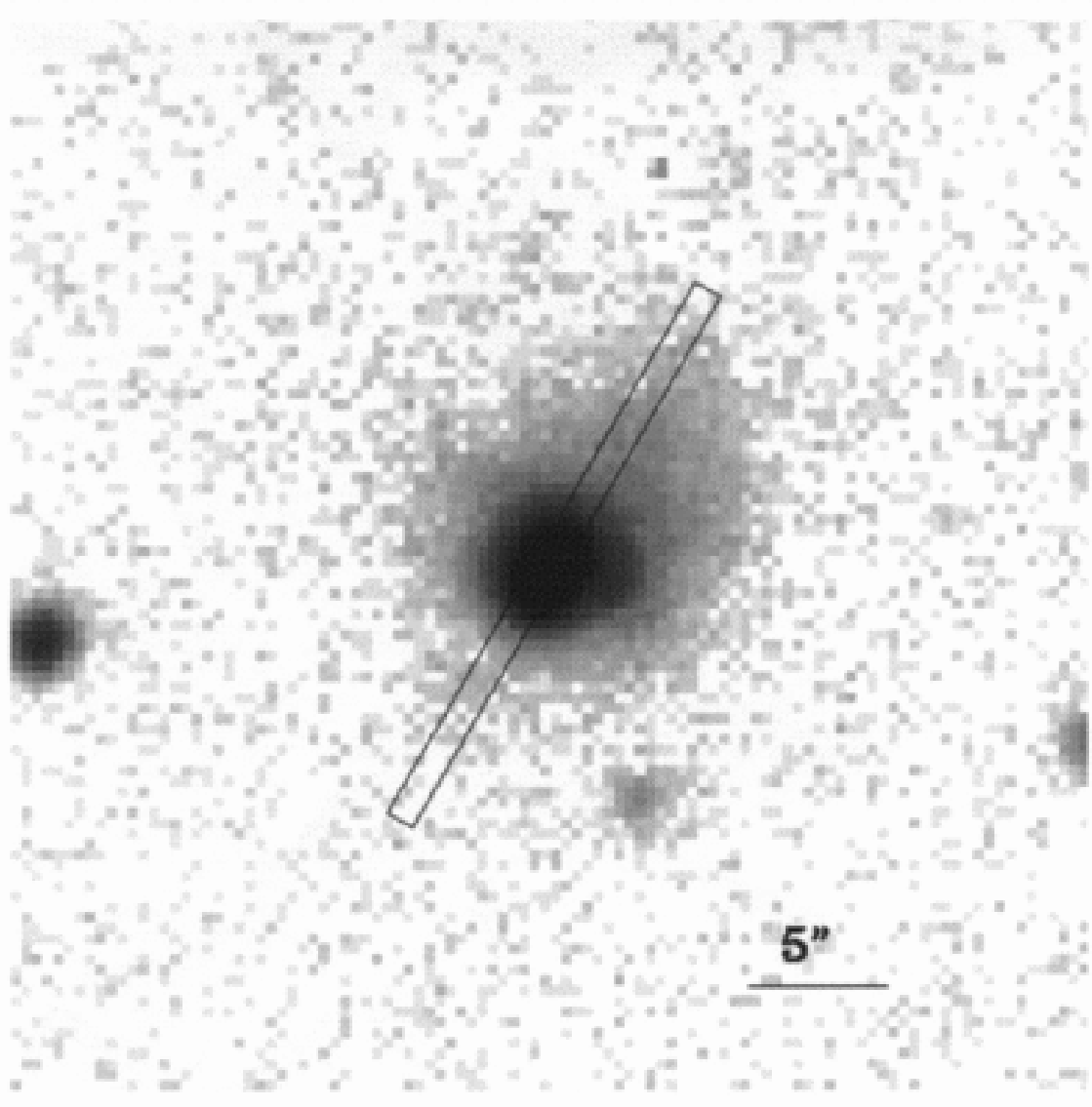
Fig. 1. from SBS 0335052, A Probable Nearby Young Dwarf Galaxy: Evidence Pro and Con Izotov et al. 1997 ApJ 476 698 doi:10.1086/303664 https://dx.doi.org/10.1086/303664 © 1997. The American Astronomical Society. All rights reserved. Printed in U.S.A.
