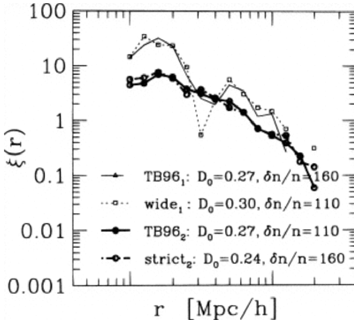
Fig. 5. from Clustering of Loose Groups and Galaxies in the PerseusPisces Survey TrasartiBattistoni, Invernizzi, & Bonometto 1997 ApJ 475 1 doi:10.1086/303523 https://dx.doi.org/10.1086/303523 © 1997. The American Astronomical Society. All rights reserved. Printed in U.S.A.
