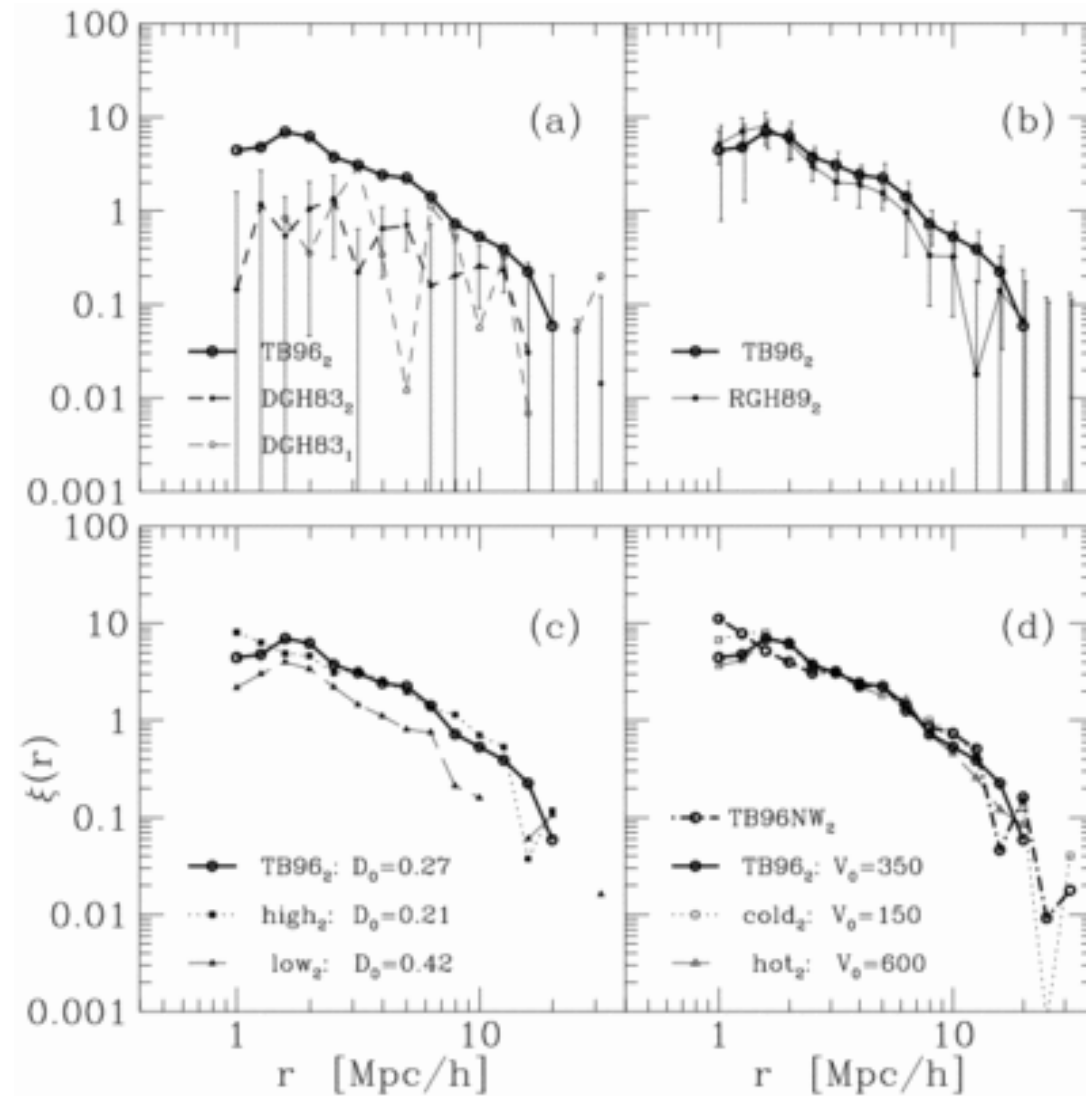
Fig. 4. from Clustering of Loose Groups and Galaxies in the PerseusPisces Survey TrasartiBattistoni, Invernizzi, & Bonometto 1997 ApJ 475 1 doi:10.1086/303523 https://dx.doi.org/10.1086/303523 © 1997. The American Astronomical Society. All rights reserved. Printed in U.S.A.
