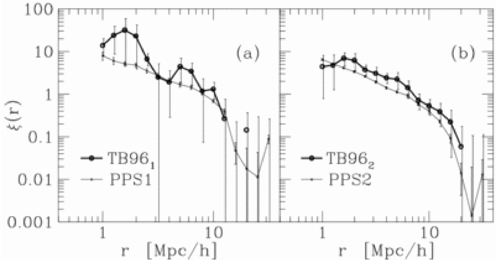
Fig. 3. from Clustering of Loose Groups and Galaxies in the PerseusPisces Survey TrasartiBattistoni, Invernizzi, & Bonometto 1997 ApJ 475 1 doi:10.1086/303523 https://dx.doi.org/10.1086/303523 © 1997. The American Astronomical Society. All rights reserved. Printed in U.S.A.
