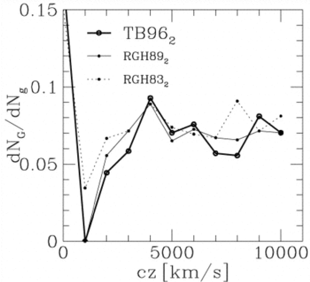
Fig. 2. from Clustering of Loose Groups and Galaxies in the PerseusPisces Survey TrasartiBattistoni, Invernizzi, & Bonometto 1997 ApJ 475 1 doi:10.1086/303523 https://dx.doi.org/10.1086/303523 © 1997. The American Astronomical Society. All rights reserved. Printed in U.S.A.
