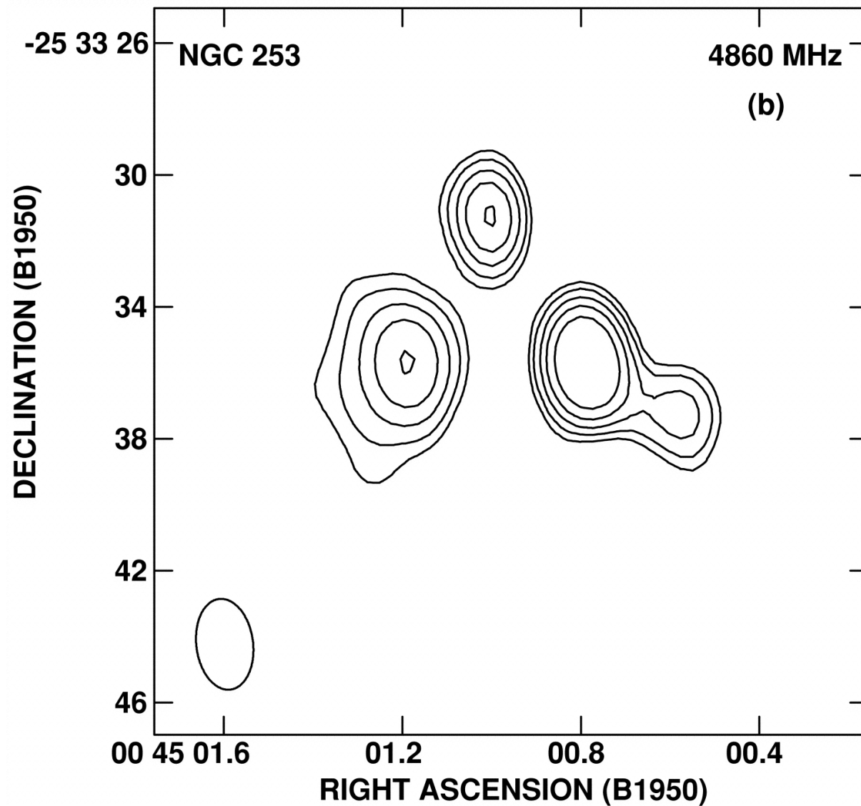
Fig. 3. from Circumnuclear Supernova Remnants and H II Regions in NGC 253 Ulvestad 2000 AJ 120 278 doi:10.1086/301428 https://dx.doi.org/10.1086/301428 © 2000. The American Astronomical Society. All rights reserved. Printed in U.S.A.
