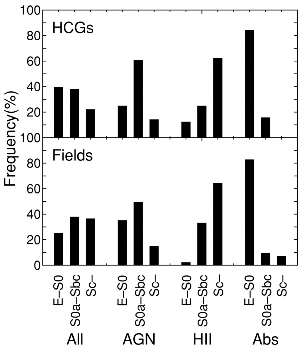
Fig. 6. from The Nuclear Activity of Galaxies in the Hickson Compact Groups Shimada et al. 2000 AJ 119 2664 doi:10.1086/301381 https://dx.doi.org/10.1086/301381 © 2000. The American Astronomical Society. All rights reserved. Printed in U.S.A.
