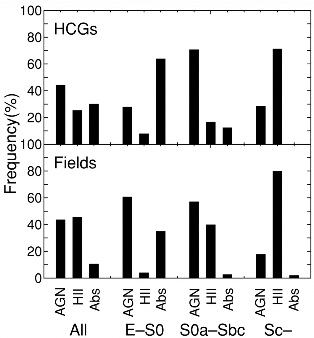
Fig. 5. from The Nuclear Activity of Galaxies in the Hickson Compact Groups Shimada et al. 2000 AJ 119 2664 doi:10.1086/301381 https://dx.doi.org/10.1086/301381 © 2000. The American Astronomical Society. All rights reserved. Printed in U.S.A.
