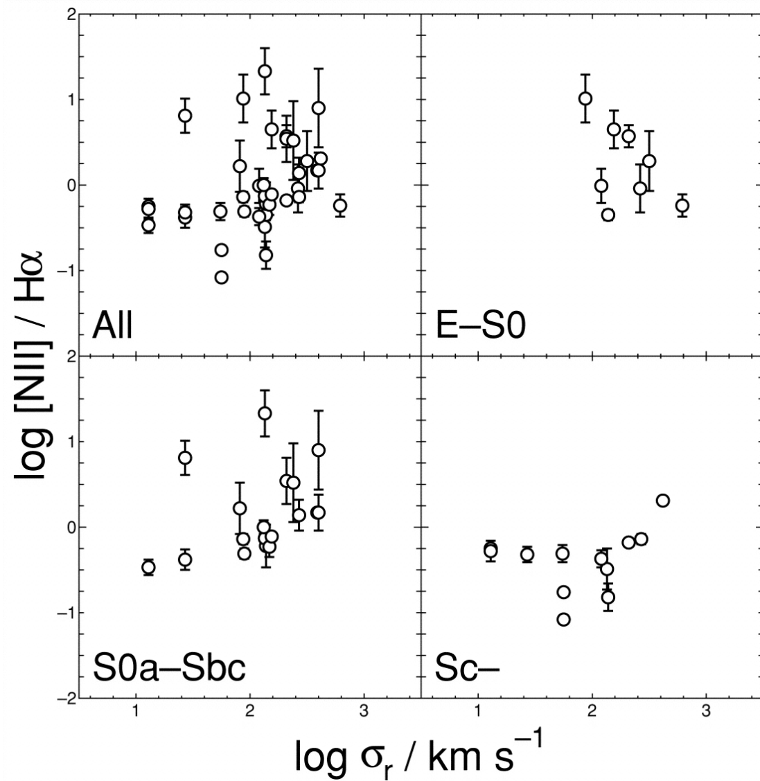
Fig. 3. from The Nuclear Activity of Galaxies in the Hickson Compact Groups Shimada et al. 2000 AJ 119 2664 doi:10.1086/301381 https://dx.doi.org/10.1086/301381 © 2000. The American Astronomical Society. All rights reserved. Printed in U.S.A.
