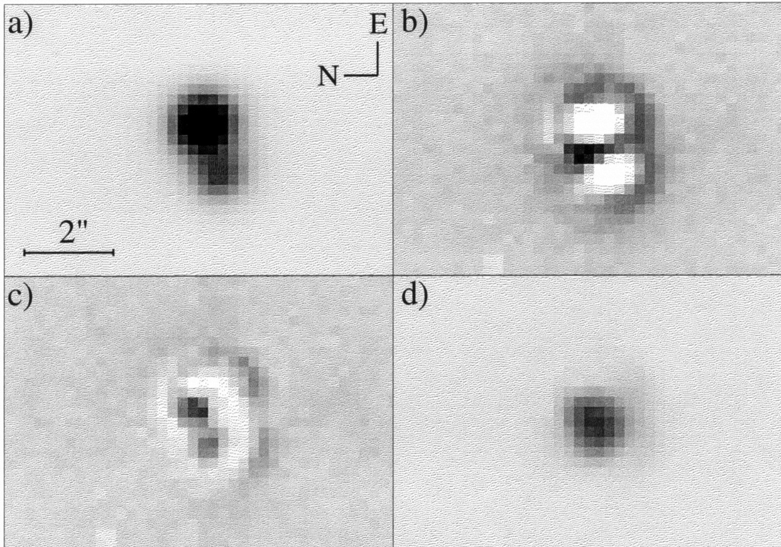
Fig. 2. from CTQ 414: A New Gravitational Lens Morgan et al. 1999 AJ 118 1444 doi:10.1086/301056 https://dx.doi.org/10.1086/301056 © 1999. The American Astronomical Society. All rights reserved. Printed in U.S.A.
