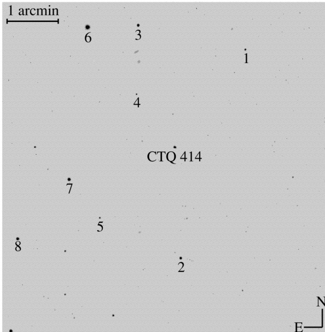
Fig. 1. from CTQ 414: A New Gravitational Lens Morgan et al. 1999 AJ 118 1444 doi:10.1086/301056 https://dx.doi.org/10.1086/301056 © 1999. The American Astronomical Society. All rights reserved. Printed in U.S.A.
