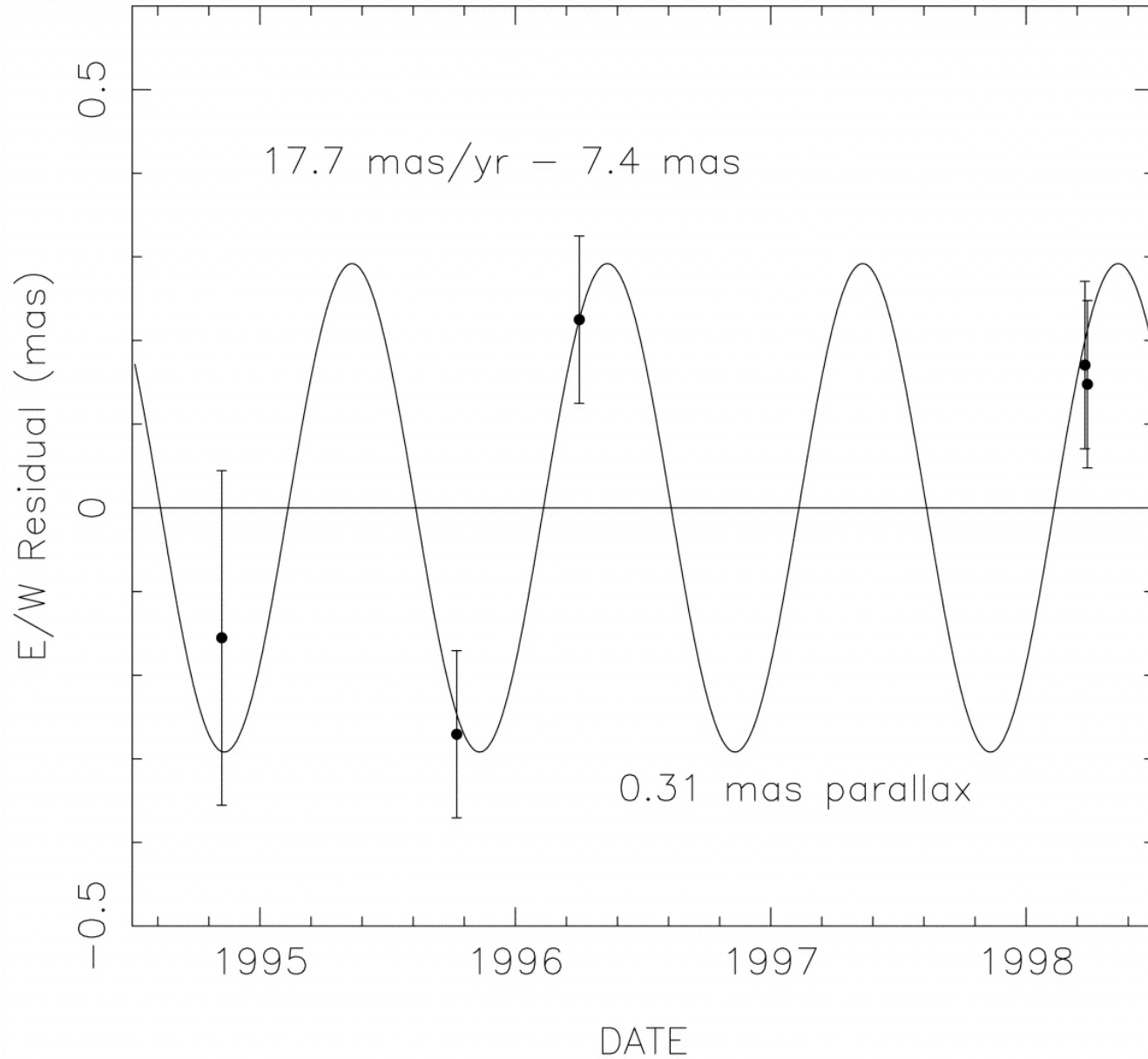
Fig. 4. from SubMilliarcsecond Precision of Pulsar Motions: Using InBeam Calibrators with the VLBA Fomalont et al. 1999 AJ 117 3025 doi:10.1086/300877 https://dx.doi.org/10.1086/300877 © 1999. The American Astronomical Society. All rights reserved. Printed in U.S.A.
