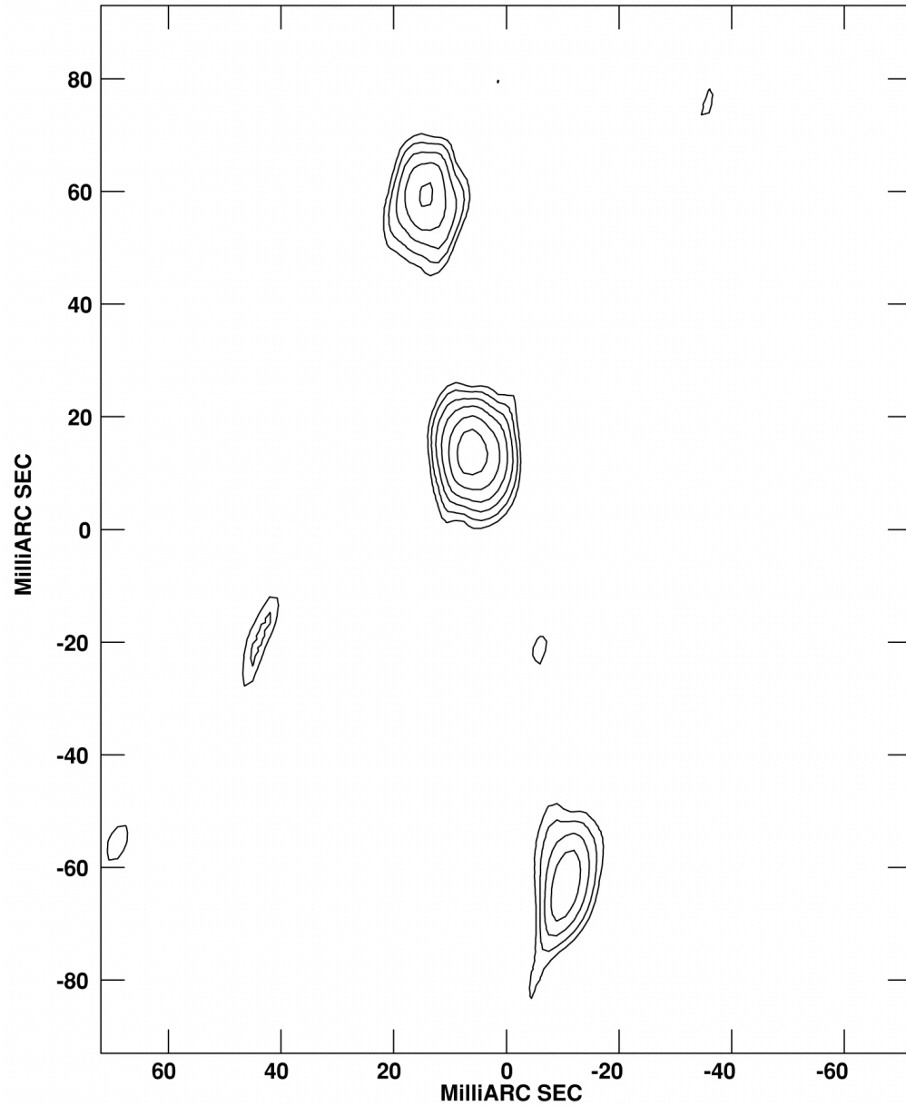
Fig. 2. from SubMilliarcsecond Precision of Pulsar Motions: Using InBeam Calibrators with the VLBA Fomalont et al. 1999 AJ 117 3025 doi:10.1086/300877 https://dx.doi.org/10.1086/300877 © 1999. The American Astronomical Society. All rights reserved. Printed in U.S.A.
