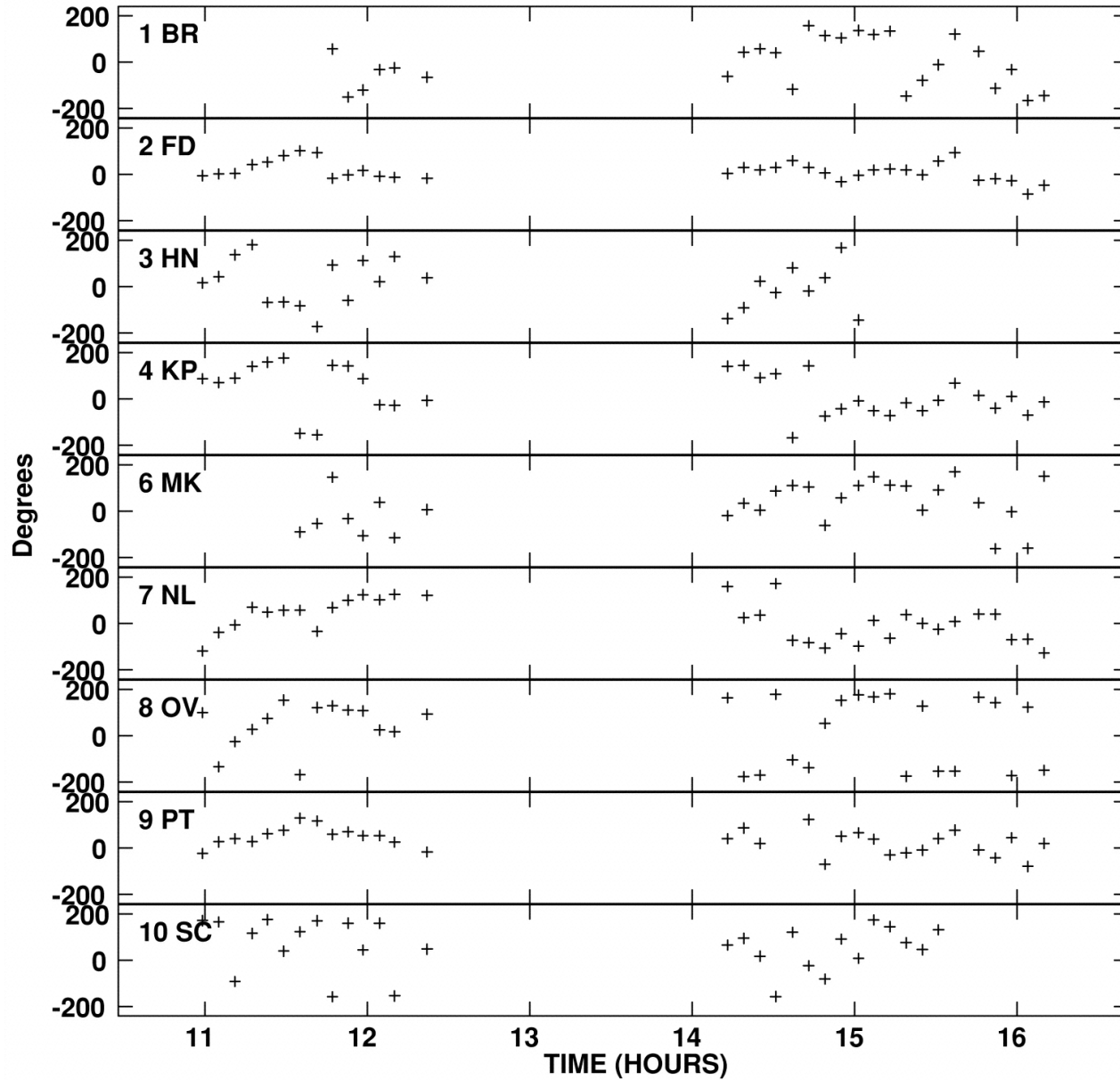
Fig. 1. from SubMilliarcsecond Precision of Pulsar Motions: Using InBeam Calibrators with the VLBA Fomalont et al. 1999 AJ 117 3025 doi:10.1086/300877 https://dx.doi.org/10.1086/300877
