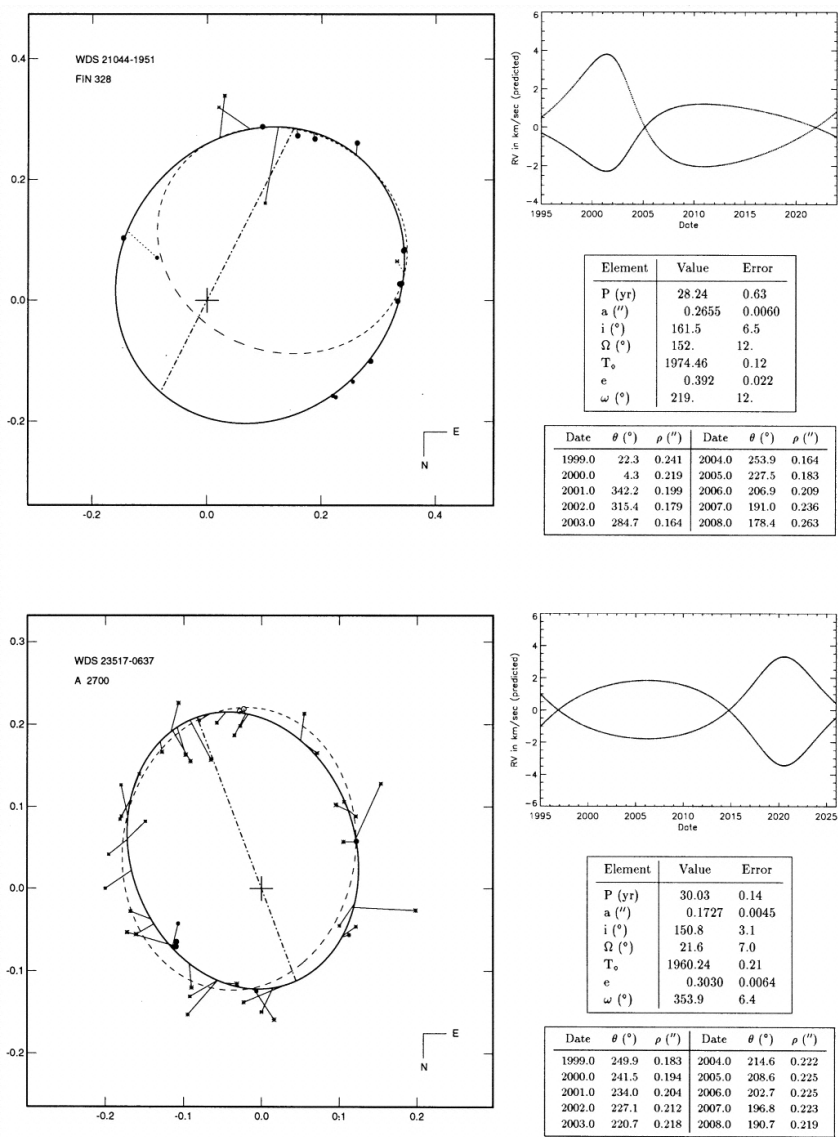
Fig. 6. from Binary Star Orbits from Speckle Interferometry. I. Improved Orbital Elements of 22 Visual Systems Mason, Douglass, & Hartkopf 1999 AJ 117 1023 doi:10.1086/300748 https://dx.doi.org/10.1086/300748 © 1999. The American Astronomical Society. All rights reserved. Printed in U.S.A.
