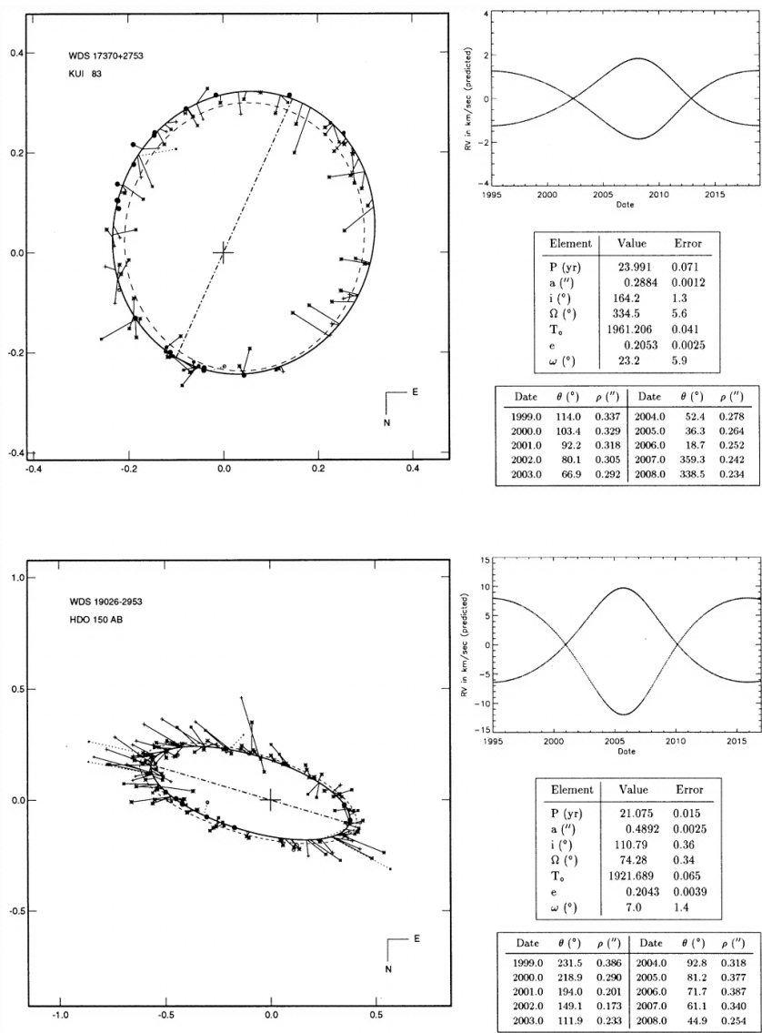
Fig. 5. from Binary Star Orbits from Speckle Interferometry. I. Improved Orbital Elements of 22 Visual Systems Mason, Douglass, & Hartkopf 1999 AJ 117 1023 doi:10.1086/300748 https://dx.doi.org/10.1086/300748 © 1999. The American Astronomical Society. All rights reserved. Printed in U.S.A.
