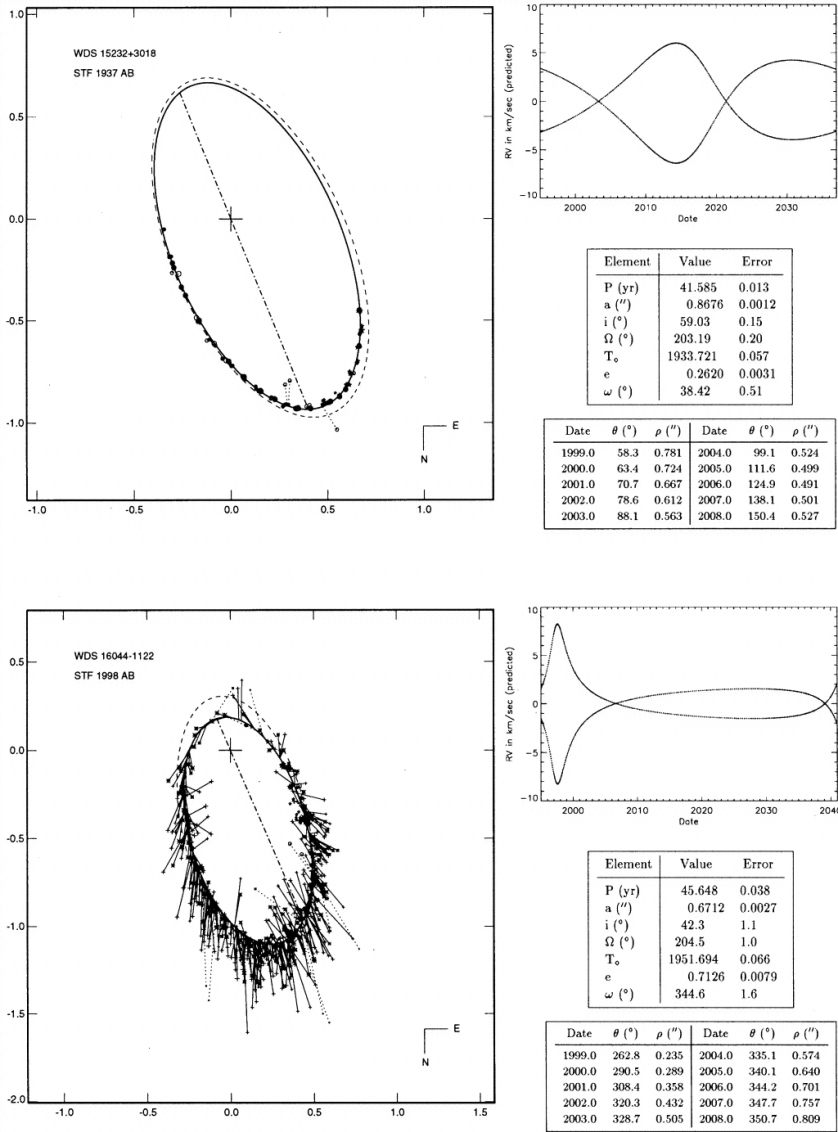
Fig. 4. from Binary Star Orbits from Speckle Interferometry. I. Improved Orbital Elements of 22 Visual Systems Mason, Douglass, & Hartkopf 1999 AJ 117 1023 doi:10.1086/300748 https://dx.doi.org/10.1086/300748 © 1999. The American Astronomical Society. All rights reserved. Printed in U.S.A.
