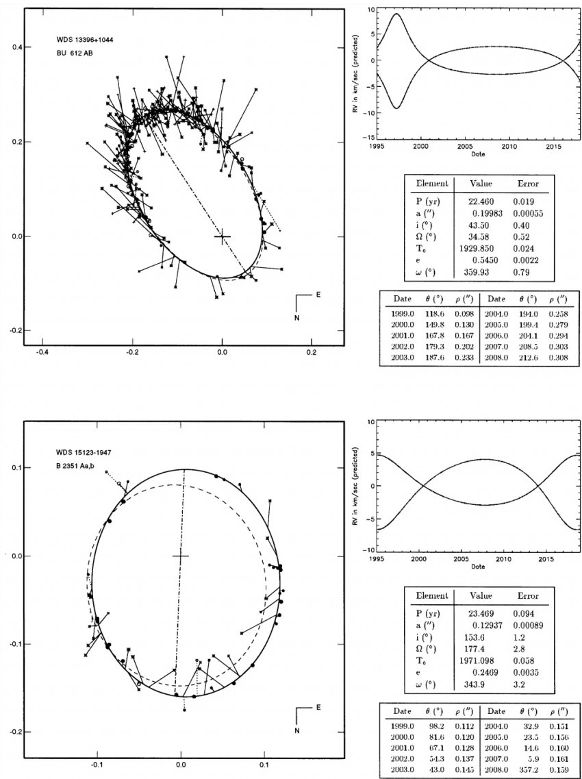
Fig. 3. from Binary Star Orbits from Speckle Interferometry. I. Improved Orbital Elements of 22 Visual Systems Mason, Douglass, & Hartkopf 1999 AJ 117 1023 doi:10.1086/300748 https://dx.doi.org/10.1086/300748 © 1999. The American Astronomical Society. All rights reserved. Printed in U.S.A.
