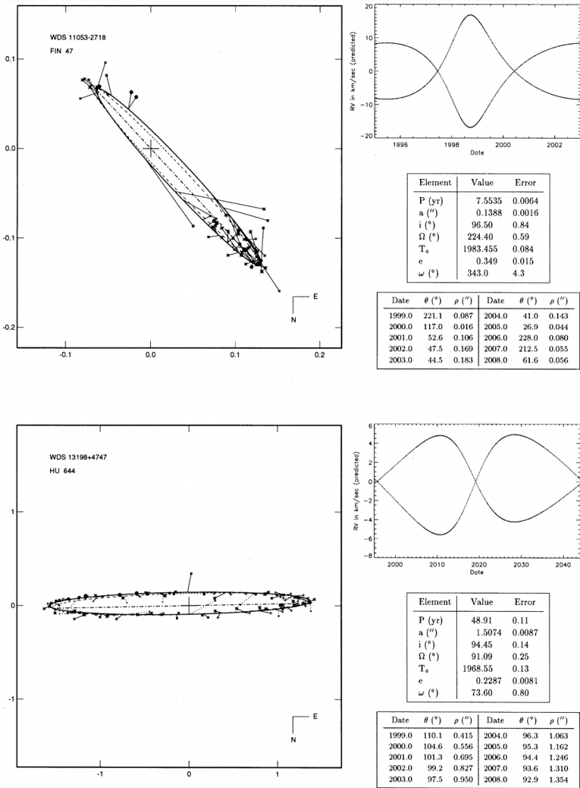
Fig. 2. from Binary Star Orbits from Speckle Interferometry. I. Improved Orbital Elements of 22 Visual Systems Mason, Douglass, & Hartkopf 1999 AJ 117 1023 doi:10.1086/300748 https://dx.doi.org/10.1086/300748 © 1999. The American Astronomical Society. All rights reserved. Printed in U.S.A.
