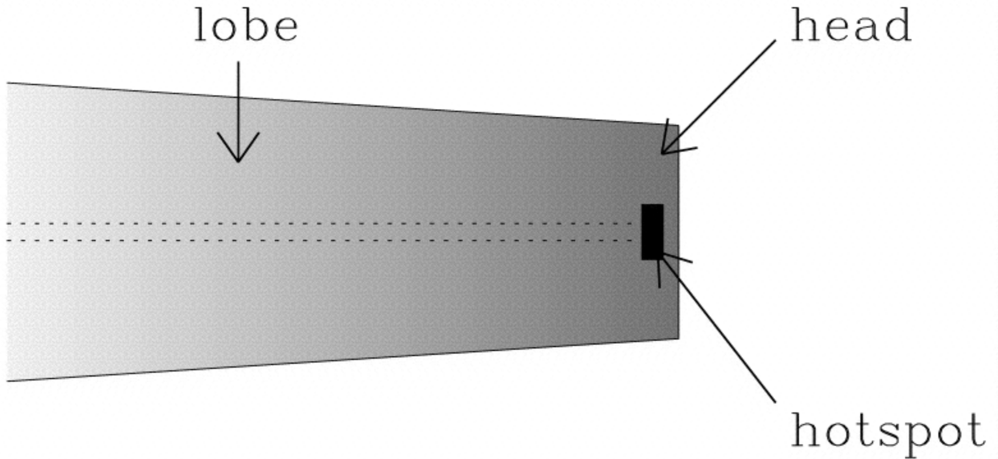
Fig. 9. from The Nature and Evolution of Classical Double Radio Sources from Complete Samples Blundell, Rawlings, & Willott 1999 AJ 117 677 doi:10.1086/300721 https://dx.doi.org/10.1086/300721 © 1999. The American Astronomical Society. All rights reserved. Printed in U.S.A.
