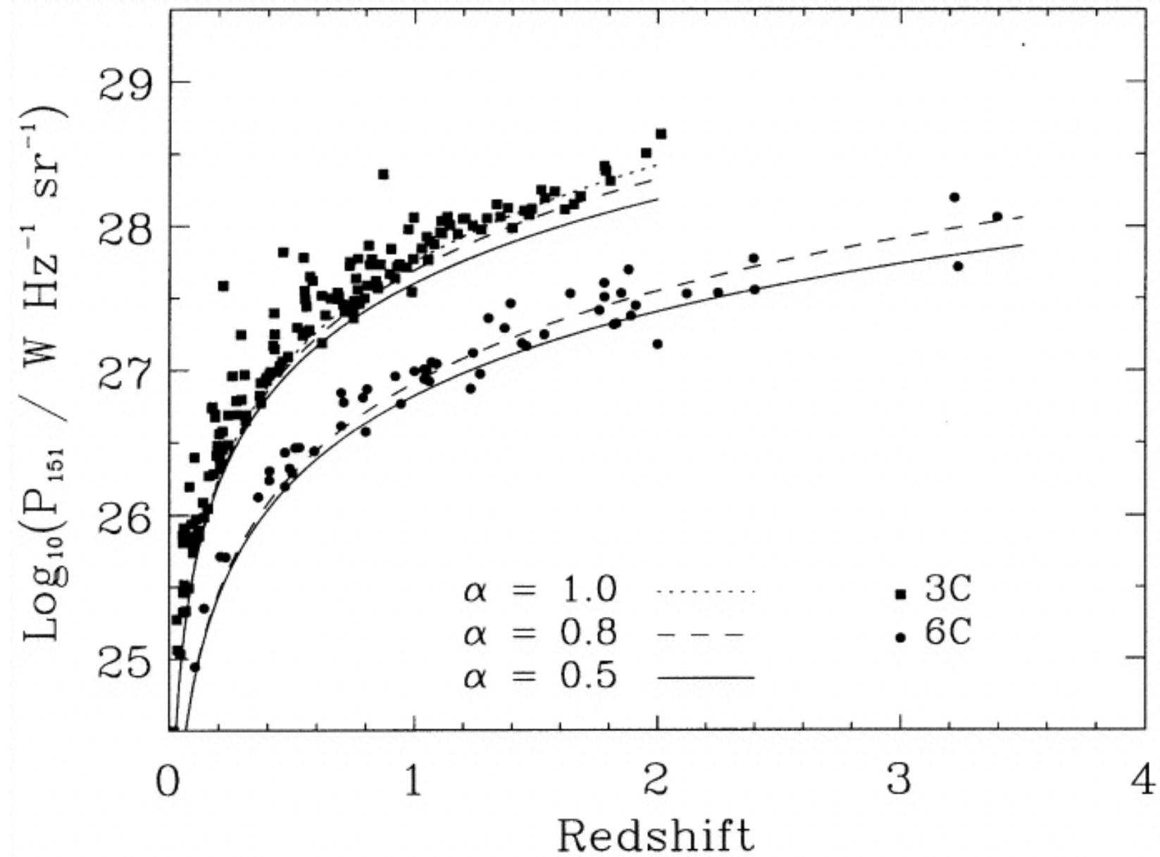
Fig. 7. from The Nature and Evolution of Classical Double Radio Sources from Complete Samples Blundell, Rawlings, & Willott 1999 AJ 117 677 doi:10.1086/300721 https://dx.doi.org/10.1086/300721 © 1999. The American Astronomical Society. All rights reserved. Printed in U.S.A.
