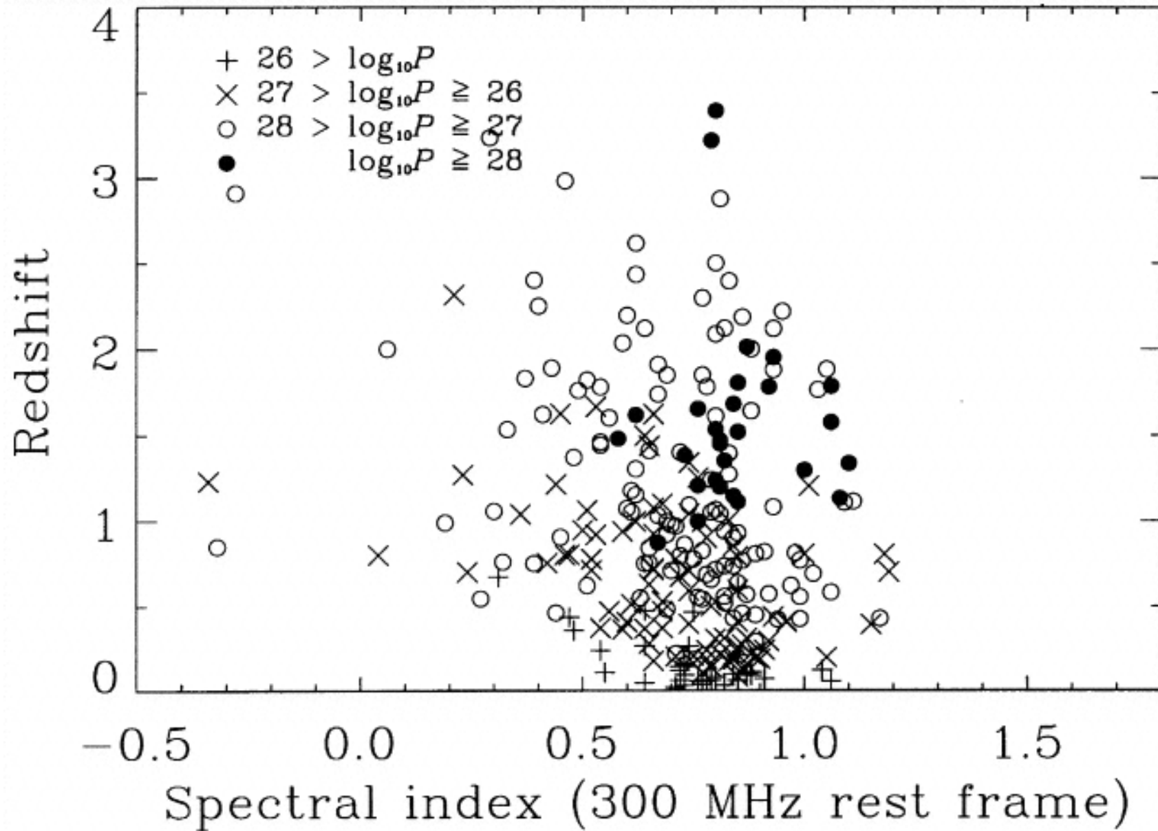
Fig. 5. from The Nature and Evolution of Classical Double Radio Sources from Complete Samples Blundell, Rawlings, & Willott 1999 AJ 117 677 doi:10.1086/300721 https://dx.doi.org/10.1086/300721 © 1999. The American Astronomical Society. All rights reserved. Printed in U.S.A.
