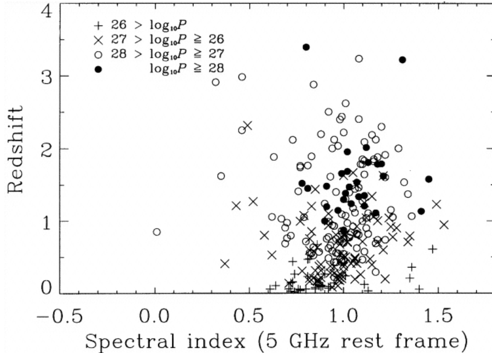
Fig. 4. from The Nature and Evolution of Classical Double Radio Sources from Complete Samples Blundell, Rawlings, & Willott 1999 AJ 117 677 doi:10.1086/300721 https://dx.doi.org/10.1086/300721
