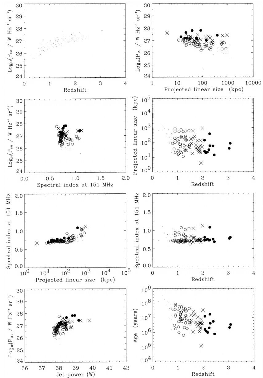
Fig. 19. from The Nature and Evolution of Classical Double Radio Sources from Complete Samples Blundell, Rawlings, & Willott 1999 AJ 117 677 doi:10.1086/300721 https://dx.doi.org/10.1086/300721
