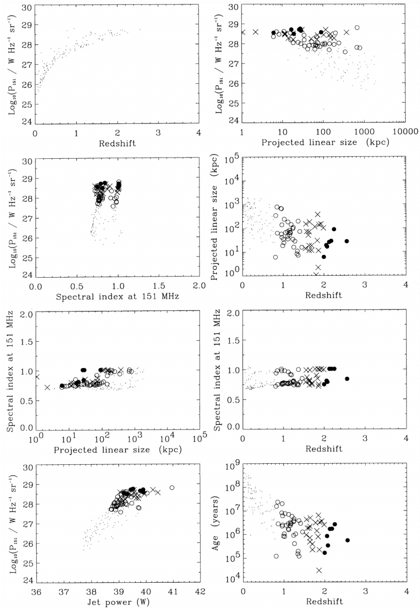
Fig. 17. from The Nature and Evolution of Classical Double Radio Sources from Complete Samples Blundell, Rawlings, & Willott 1999 AJ 117 677 doi:10.1086/300721 https://dx.doi.org/10.1086/300721
