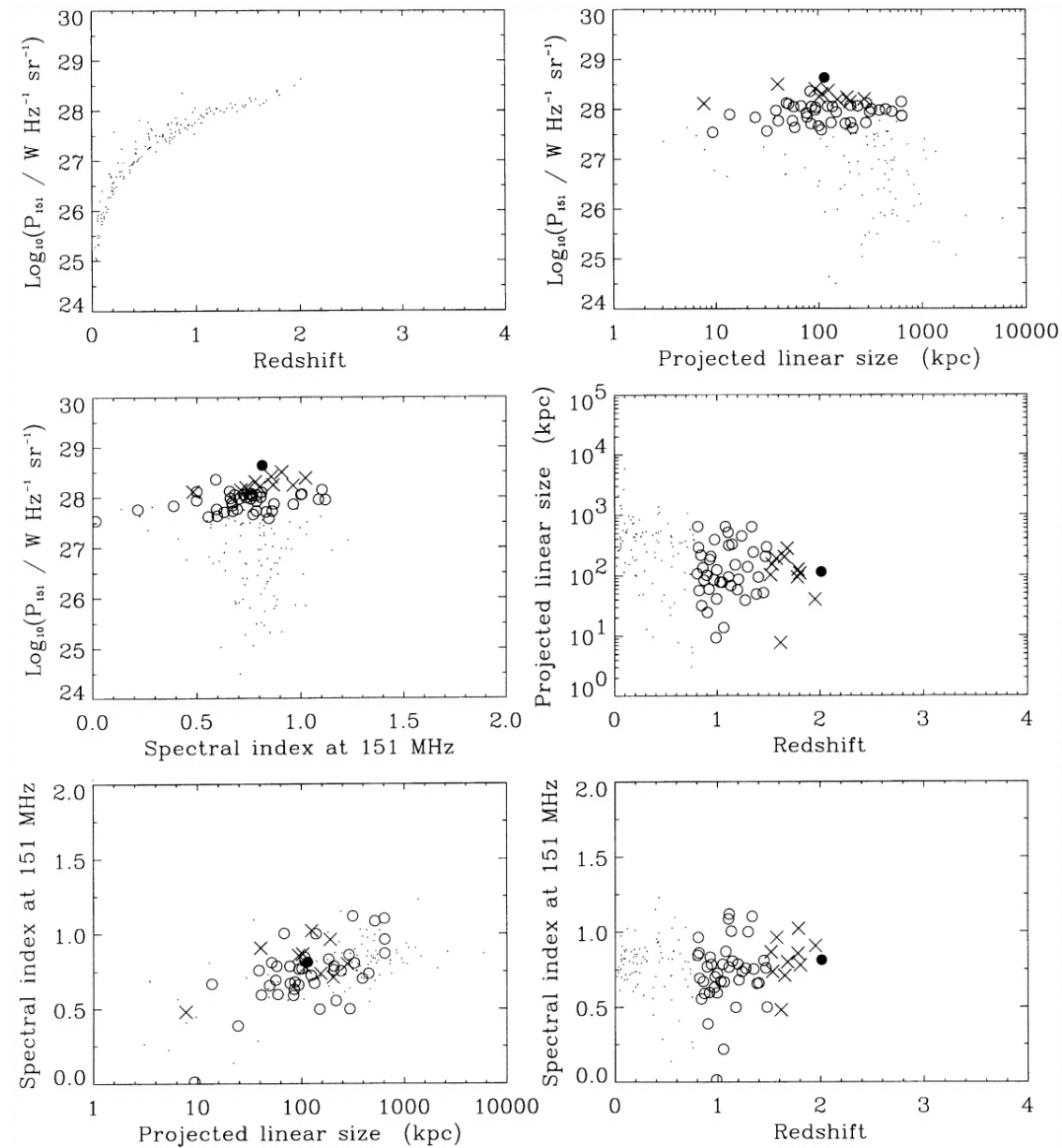
Fig. 16. from The Nature and Evolution of Classical Double Radio Sources from Complete Samples Blundell, Rawlings, & Willott 1999 AJ 117 677 doi:10.1086/300721 https://dx.doi.org/10.1086/300721
