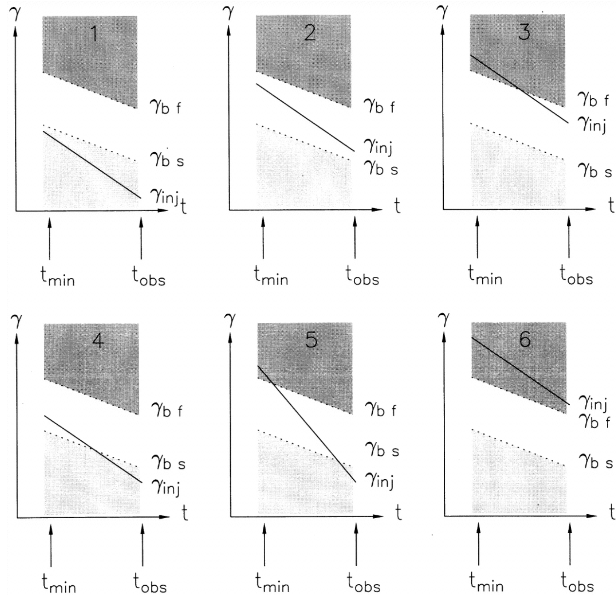
Fig. 12. from The Nature and Evolution of Classical Double Radio Sources from Complete Samples Blundell, Rawlings, & Willott 1999 AJ 117 677 doi:10.1086/300721 https://dx.doi.org/10.1086/300721
