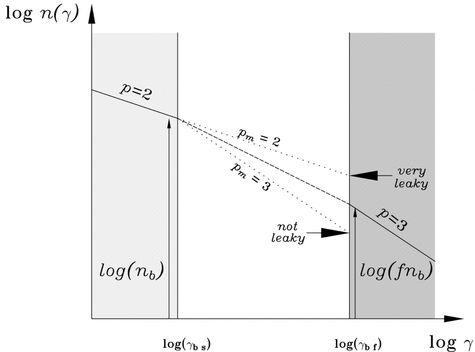
Fig. 11. from The Nature and Evolution of Classical Double Radio Sources from Complete Samples Blundell, Rawlings, & Willott 1999 AJ 117 677 doi:10.1086/300721 https://dx.doi.org/10.1086/300721 © 1999. The American Astronomical Society. All rights reserved. Printed in U.S.A.
