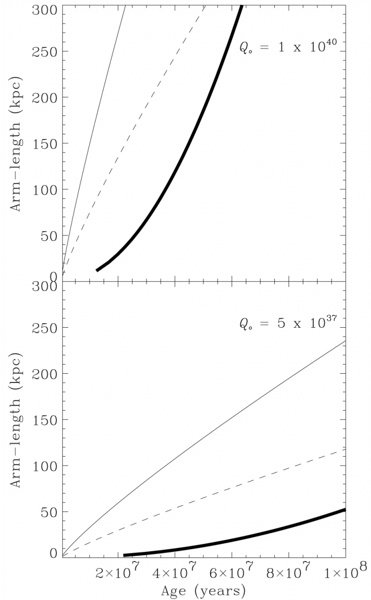
Fig. 10. from The Nature and Evolution of Classical Double Radio Sources from Complete Samples Blundell, Rawlings, & Willott 1999 AJ 117 677 doi:10.1086/300721 https://dx.doi.org/10.1086/300721
