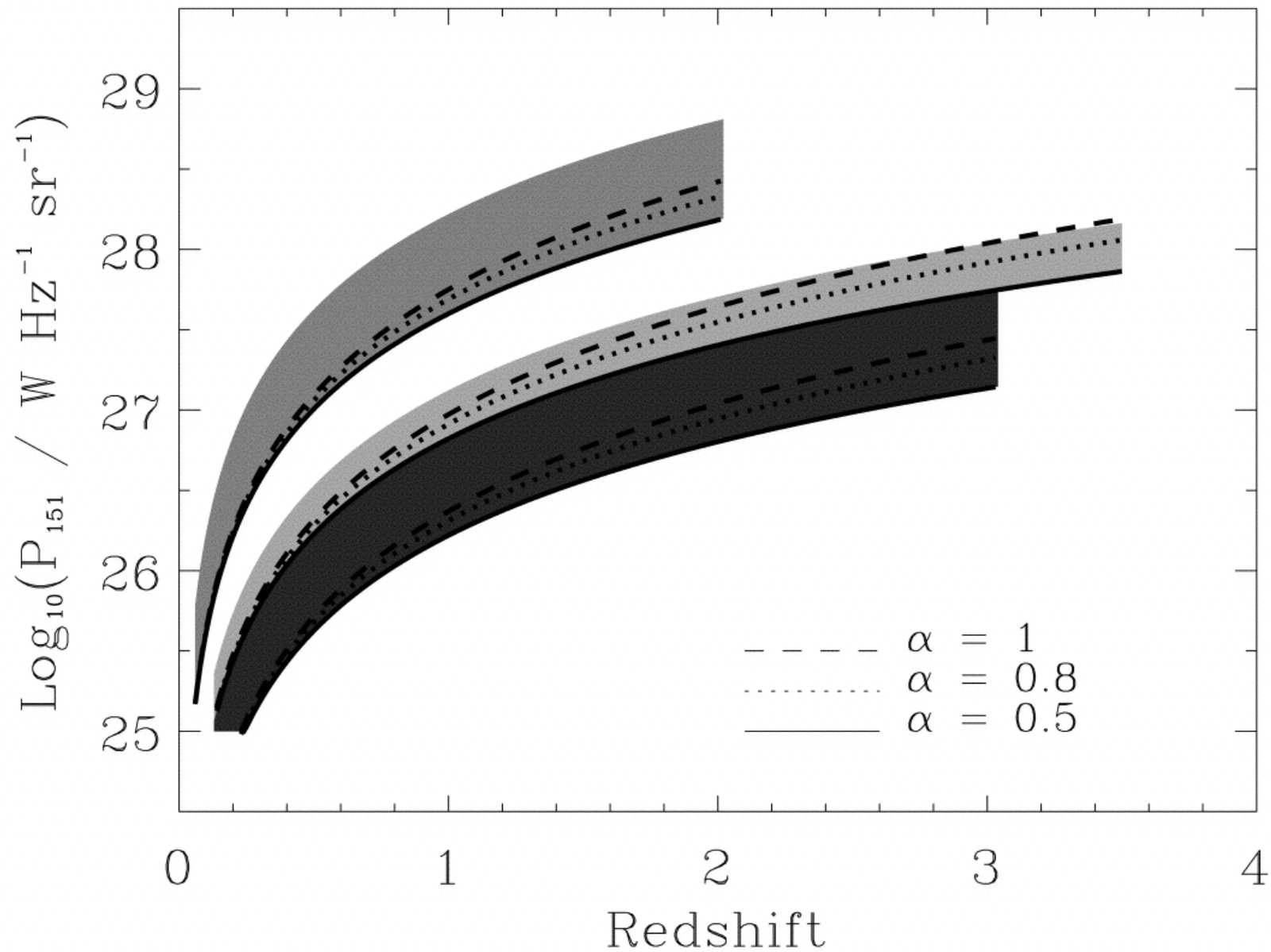
Fig. 1. from The Nature and Evolution of Classical Double Radio Sources from Complete Samples Blundell, Rawlings, & Willott 1999 AJ 117 677 doi:10.1086/300721 https://dx.doi.org/10.1086/300721 © 1999. The American Astronomical Society. All rights reserved. Printed in U.S.A.
