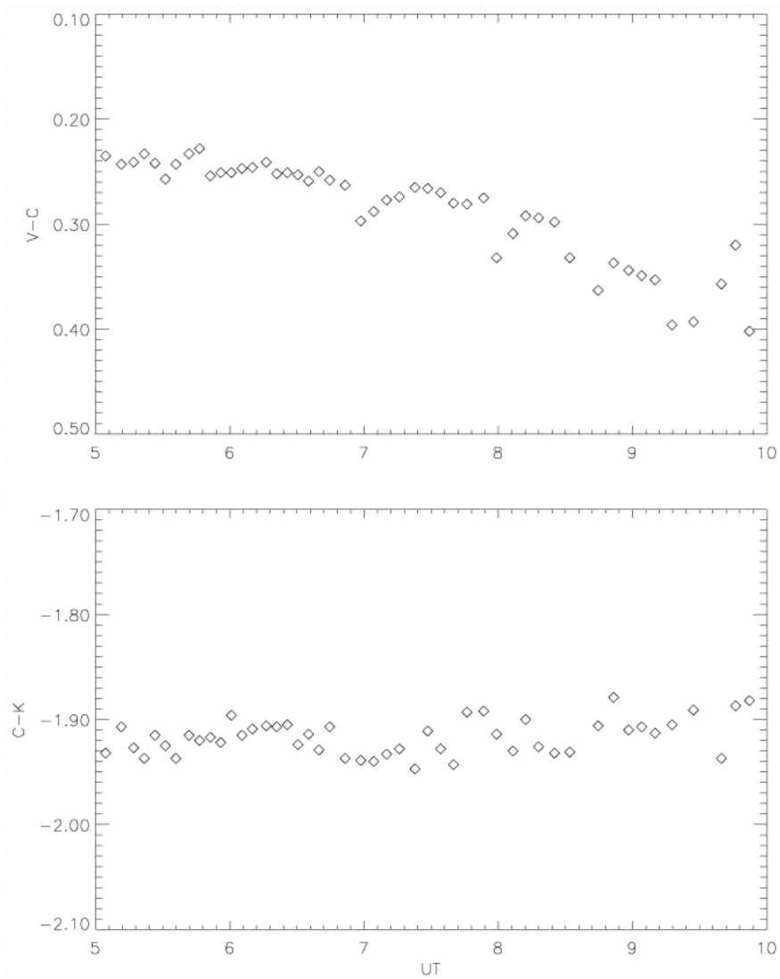
Fig. 5. from The Timescales of the Optical Variability of Blazars. V. 3C 371 Carini, Noble, & Miller 1998 AJ 116 2667 doi:10.1086/300656 https://dx.doi.org/10.1086/300656 © 1998. The American Astronomical Society. All rights reserved. Printed in U.S.A.
